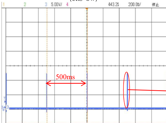
Short Circuit V_{in}=12V , Freq=2Hz (CH3=SW)
