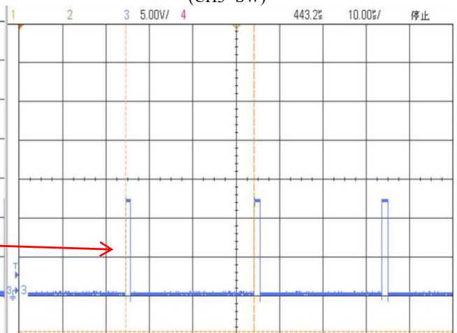
Short Circuit V_{in}=12V , Freq=34kHz (CH3=SW)
