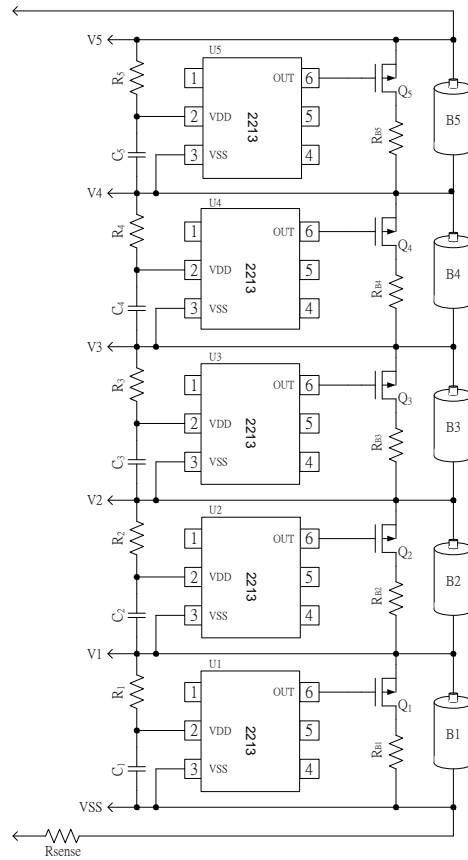
Example application of ZCC 2213-xxxB using P-MOSFET of charge balance
