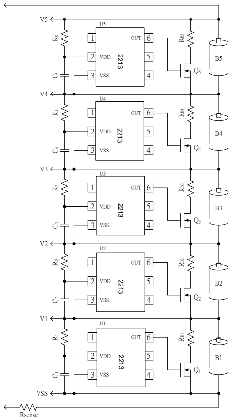
Example application of ZCC2213 xxxA using N-MOSFET of charge balance
