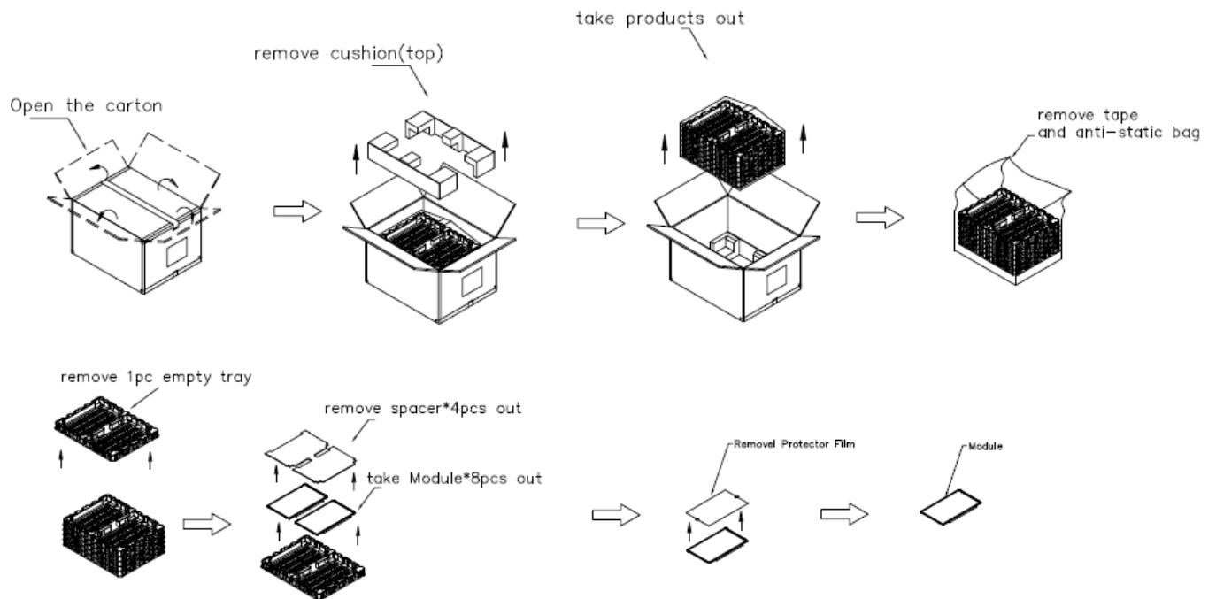
Figure. 7.4 Un-packing method
