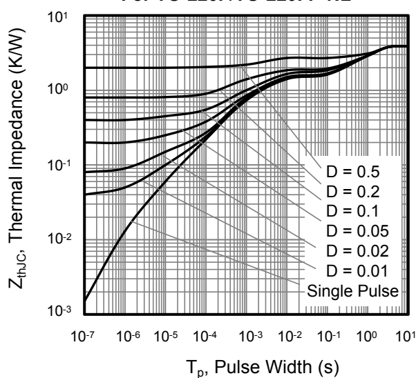
Figure 10. Transient Thermal Impedance For TO-220F/TO-220FP-NL
