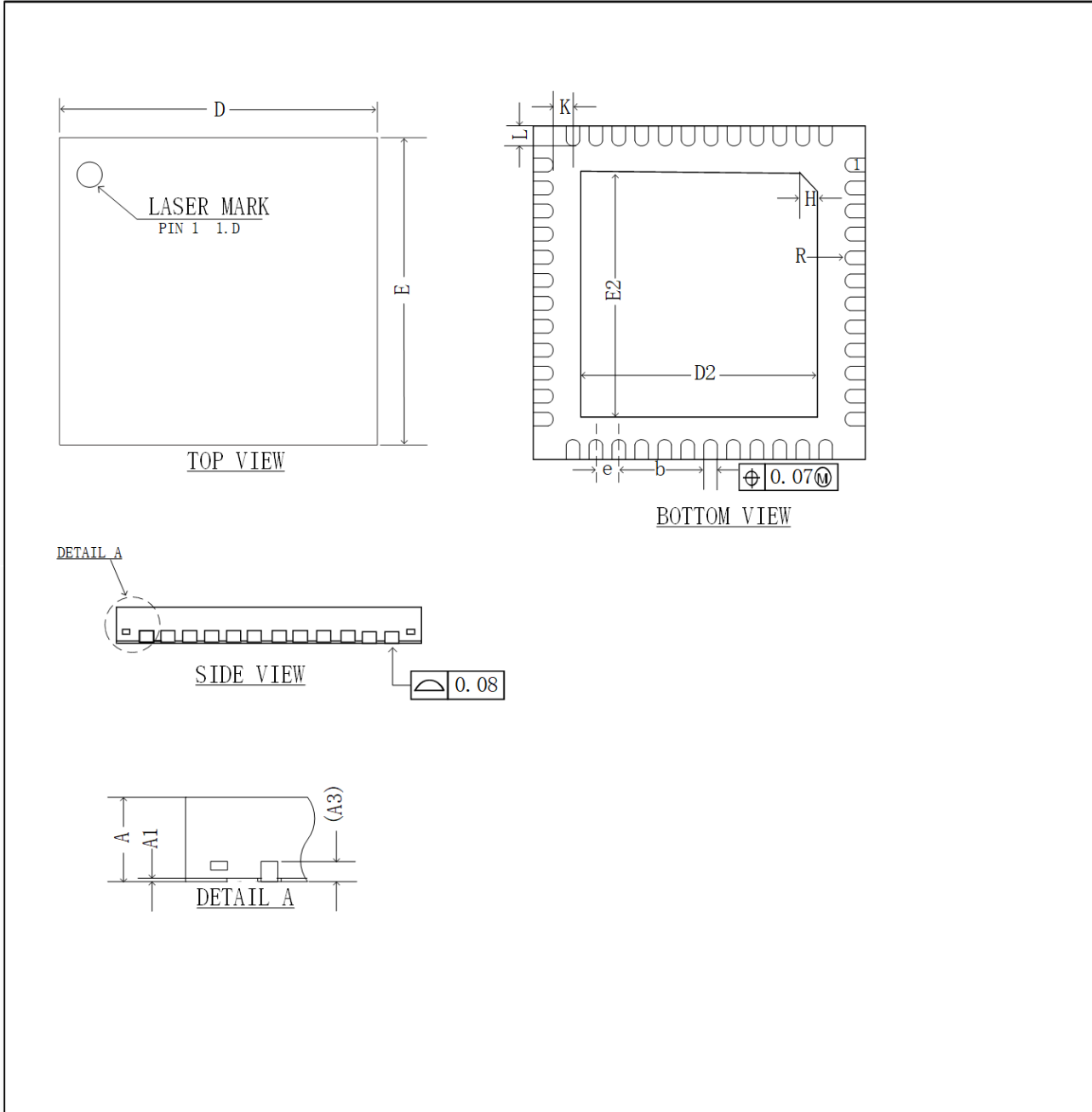
Figure 19 QFN48, 48-pin low-profile square flat package
