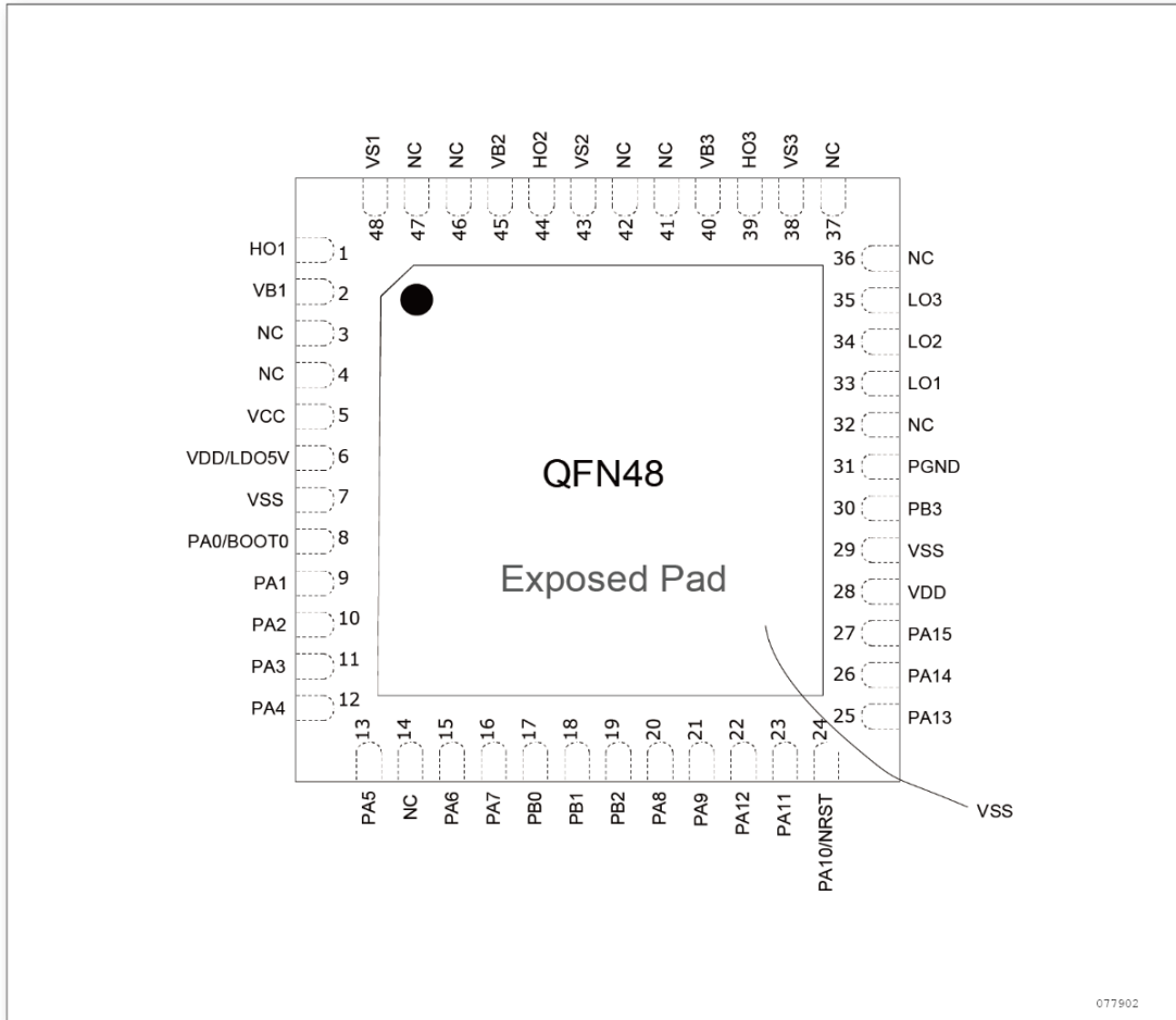
Figure 5 QFN48 pinout diagram
