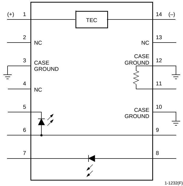
Figure 1. A1112 Laser Positive Bias Ciicuit Schematic
