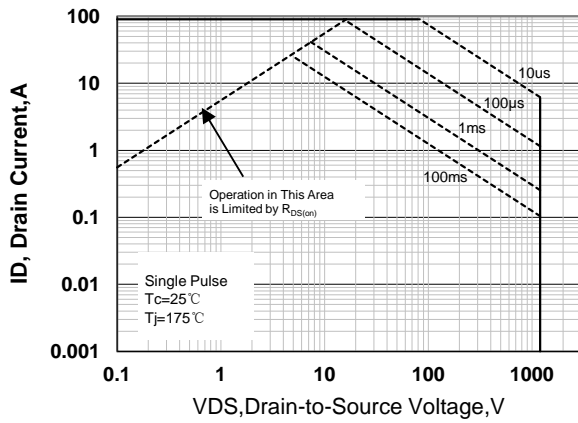
Fig 15: Safe Operating Area
