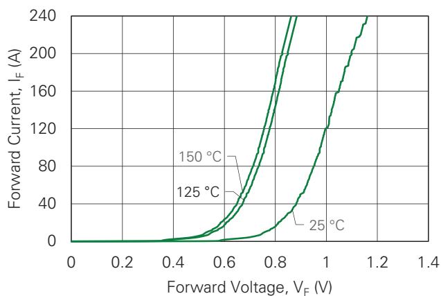
Figure 1. Maximum Forward Characteristics
