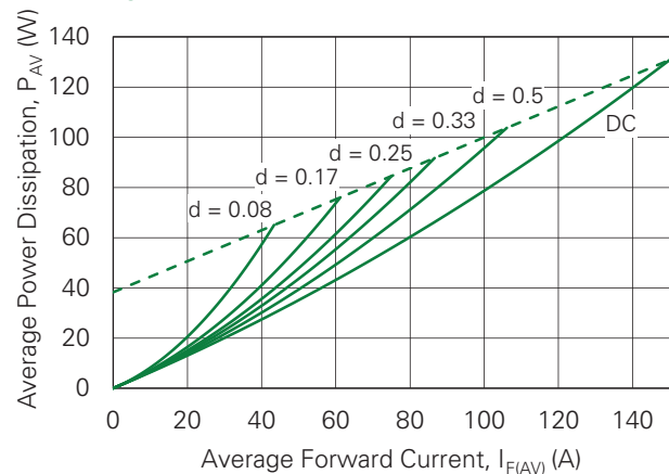
Figure 5. Forward Power Loss Characteristics
