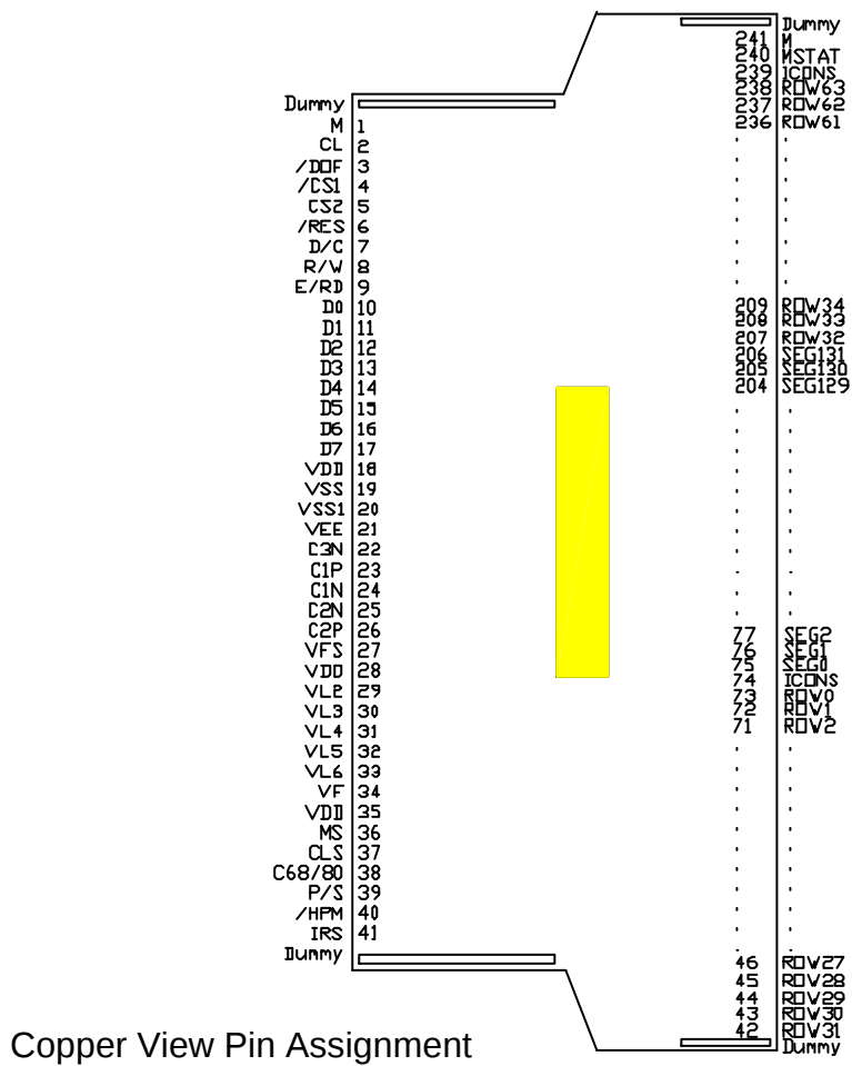
Figure 19 SSD1815T TAB Drawing 2/2
