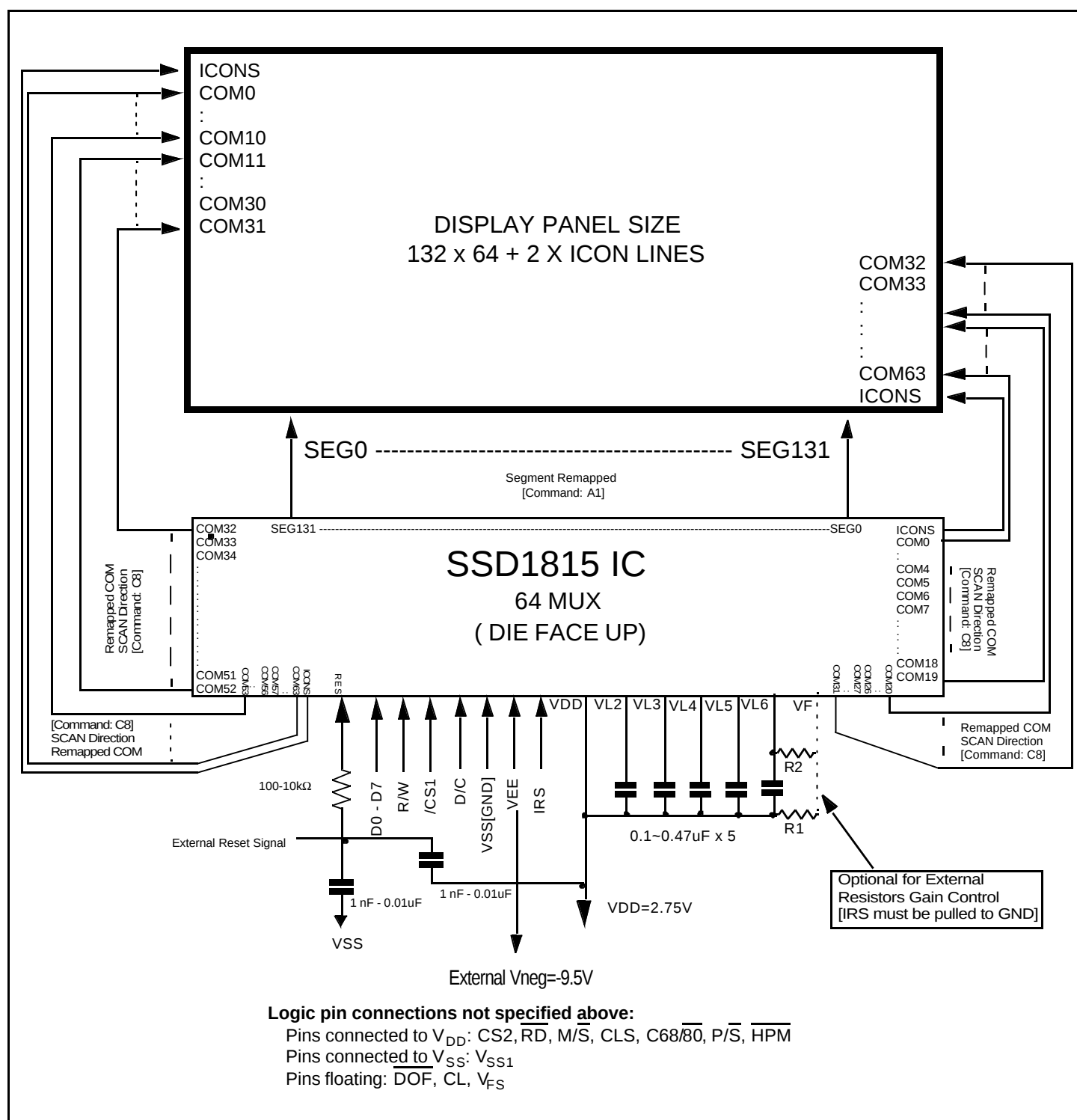
Figure 14 Application Circuit of 132 x 64 plus 2 icon lines using SSD1815, configured with: external V EE , internal regulator, divider mode enabled (Command: 2B), 6800-series MPU parallel interface, internal oscillator and master mode.
