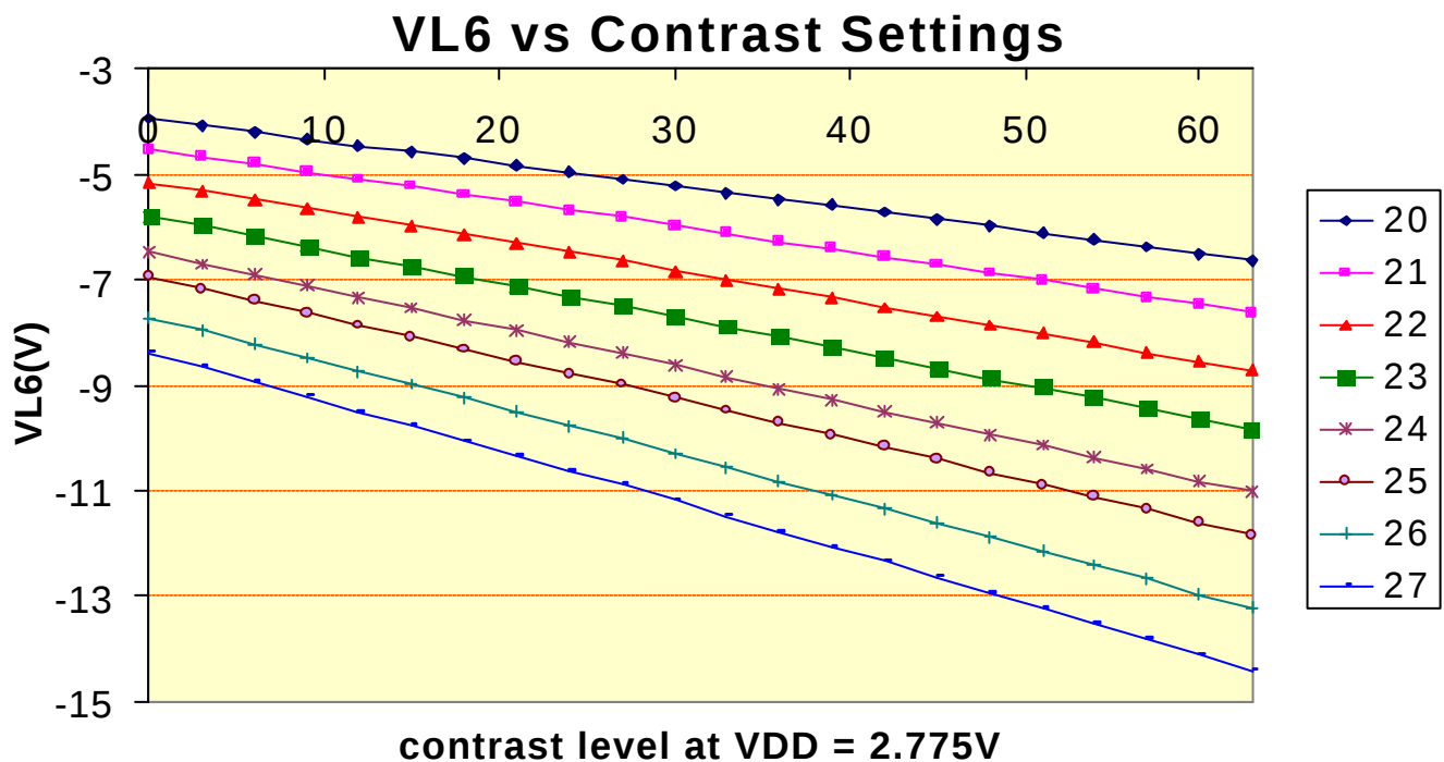
Figure 6 Voltage Regulator Output for Different Gain/Contrast Settings
