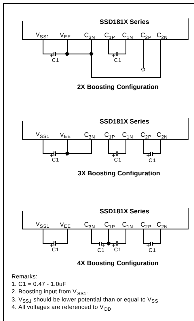
Figure 5 DC-DC Converter Configurations
