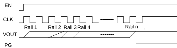
Figure 7: Soft Start when CLK Does Not Pull Down (Not Pausing)
