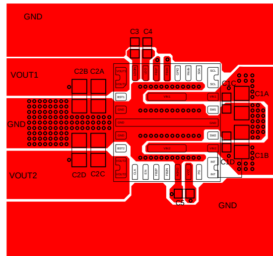
Figure 17: Recommended PCB Layout (Placement and Top Layer)
