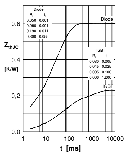
Fig. 9 Transient thermal resistance junction to case
