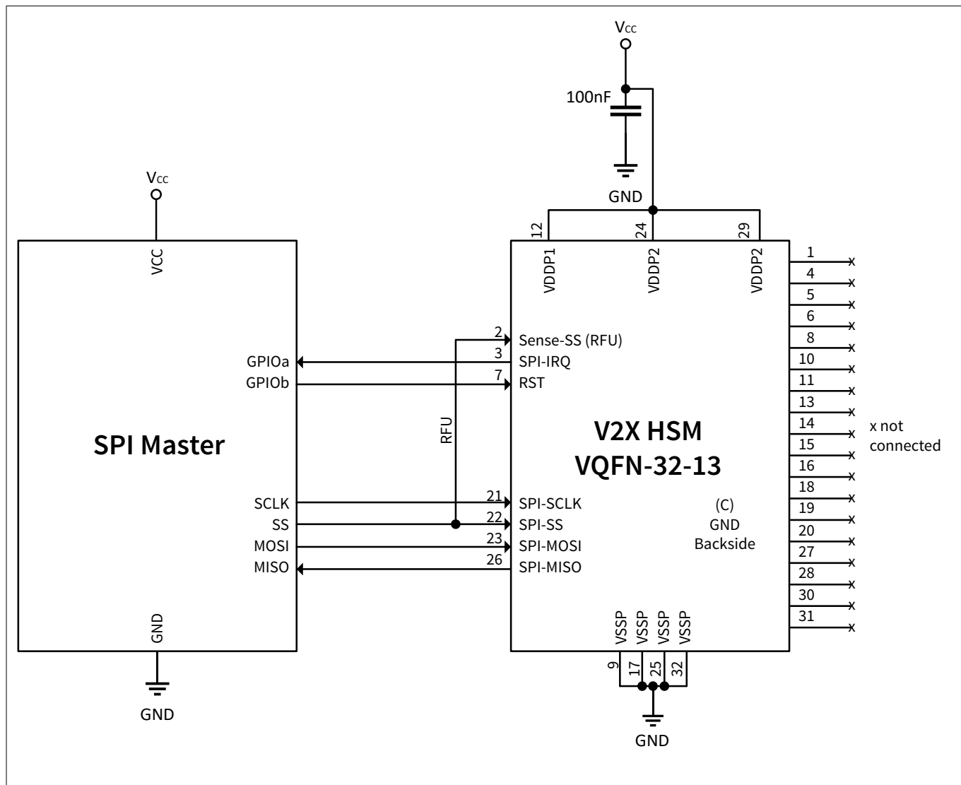
Figure 6 Typical schematic
