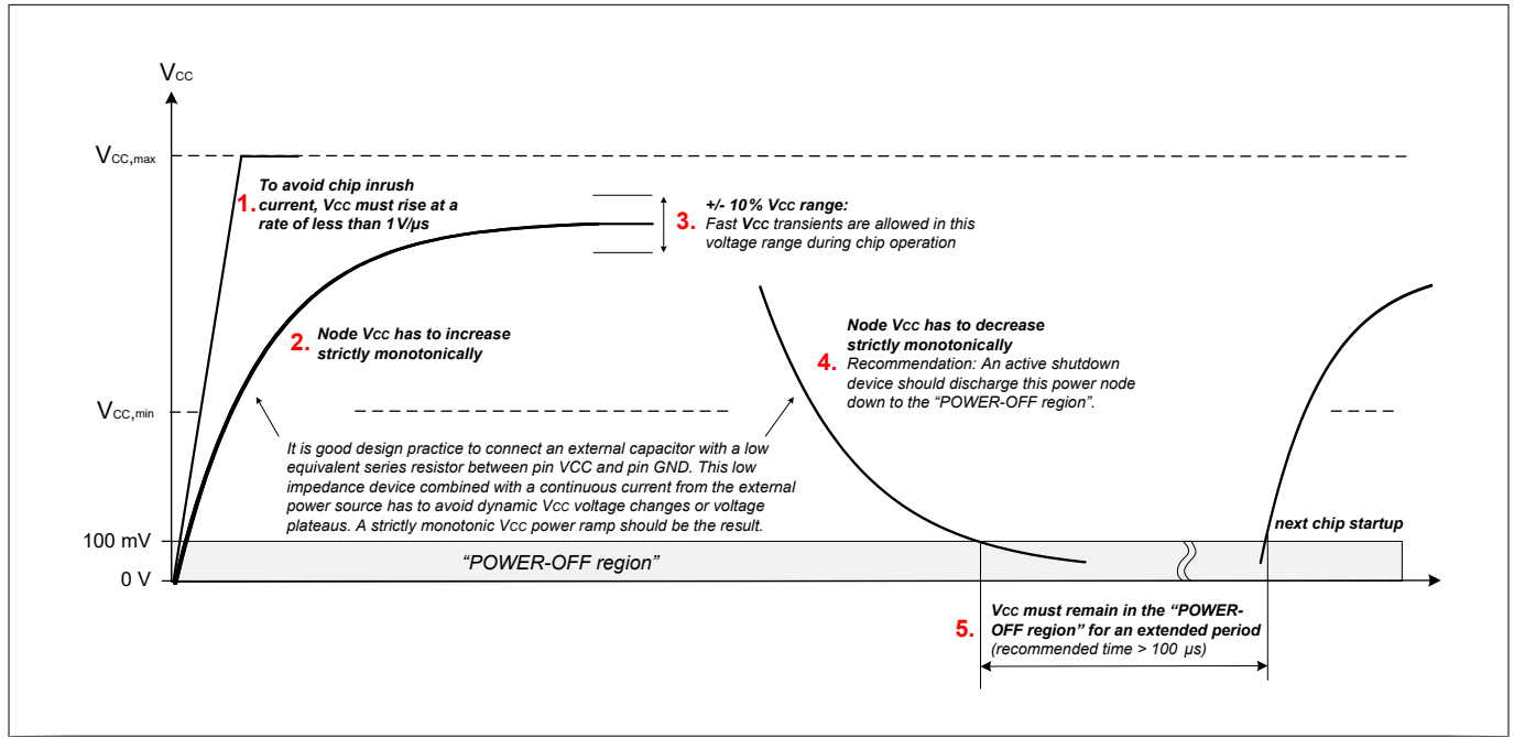
Figure 7 Recommended power-up behavior
