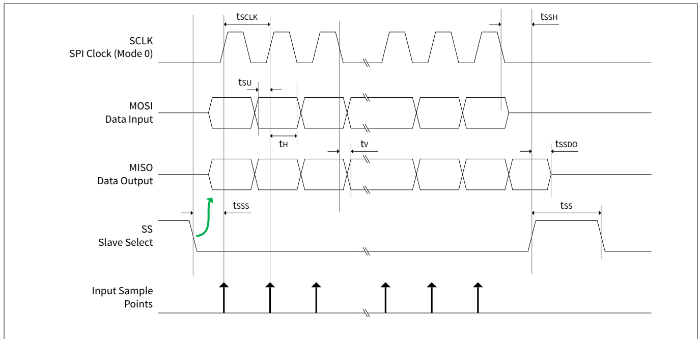
Figure 8 SPI Mode 0
