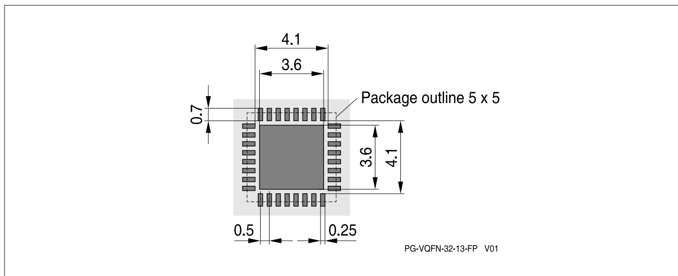
Figure 11 PG-VQFN-32-13 package footprint
