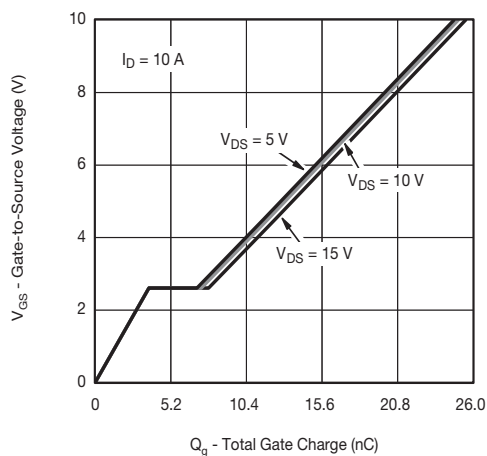
Gate Charge
