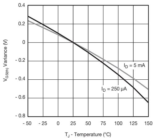
Threshold Voltage
