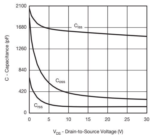
Capacitance
