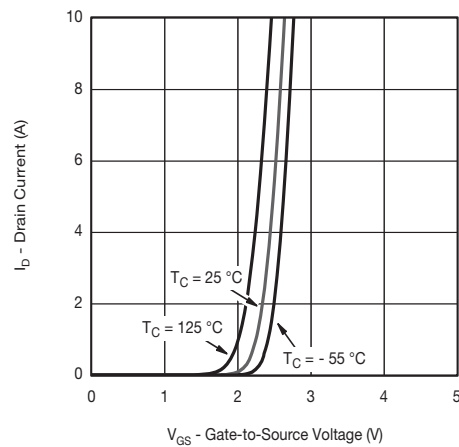
Transfer Characteristics
