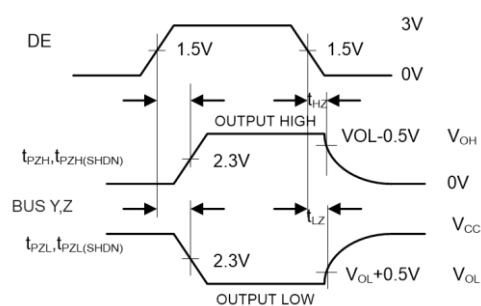
Figure 3B. Measurement Points
