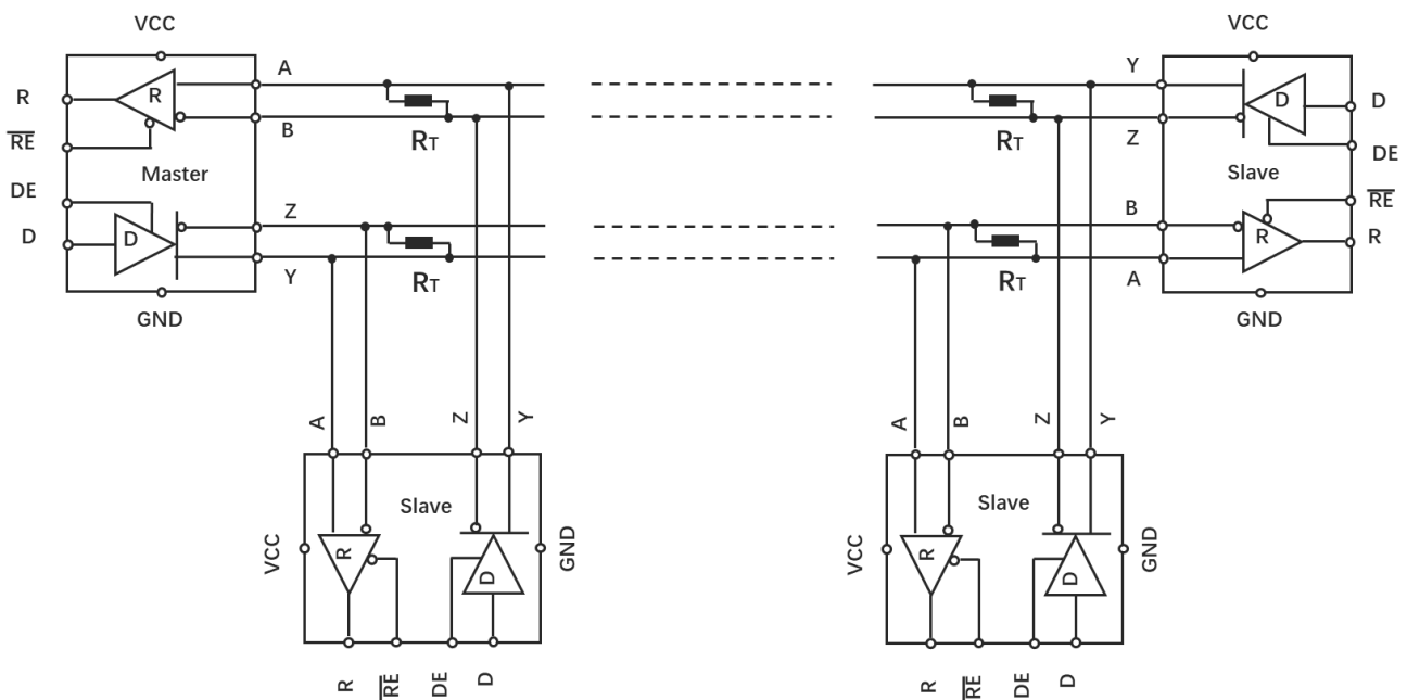
Figure 8. Typical RS485 communication network with enable function
