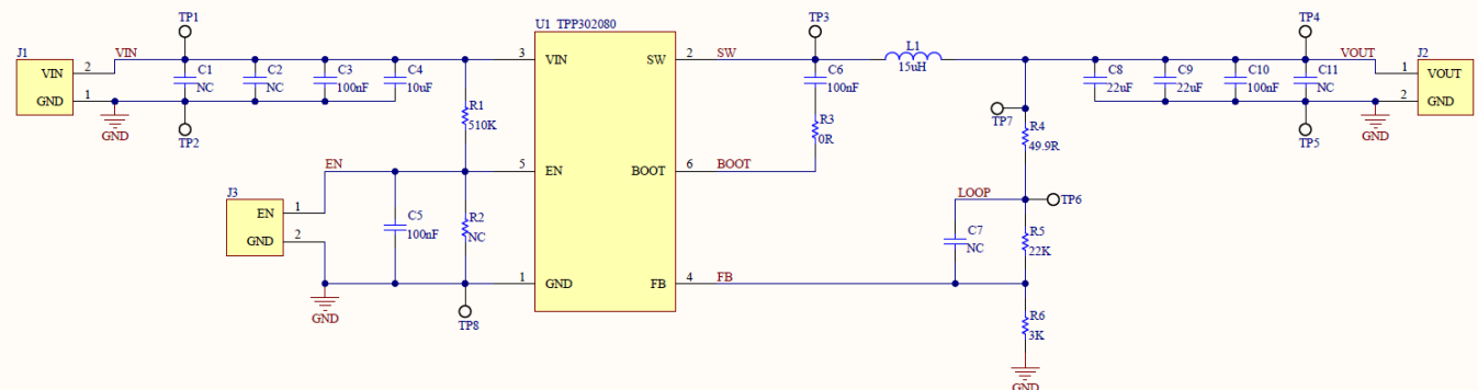
Figure 26. Typical Application Circuit
