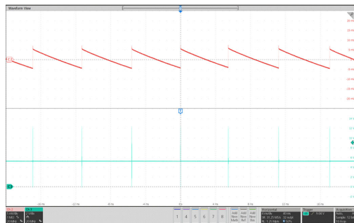
Figure 15. Pulse Skip Mode Output Voltage Ripple
