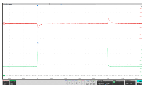
Figure 20. Load Transient
