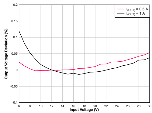
Figure 14. Line Regulation
