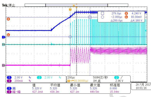
图 4, 48Vin/3LEDs (CH1:VDD CH2:VgATE CH3:Iout)
