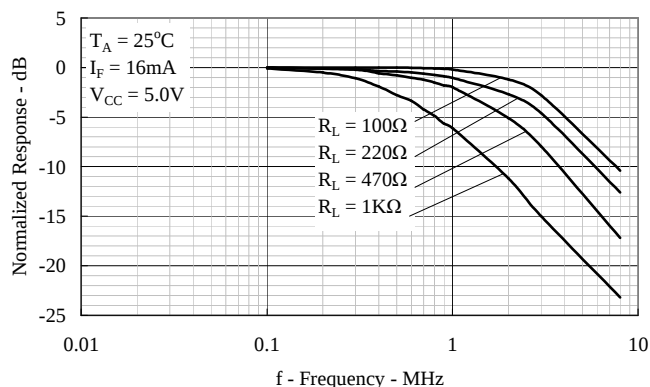
Figure 8: Frequency Response.
