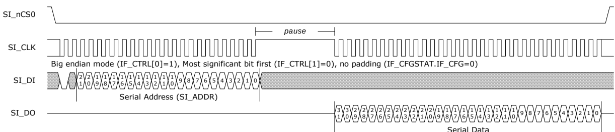
Figure 95 • Read Sequence for SI_CLK Pause
