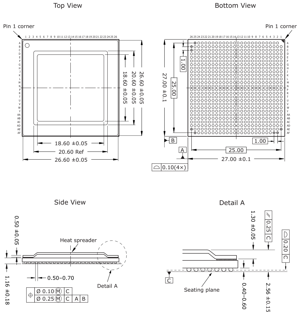
Figure 149 • Package Drawing
