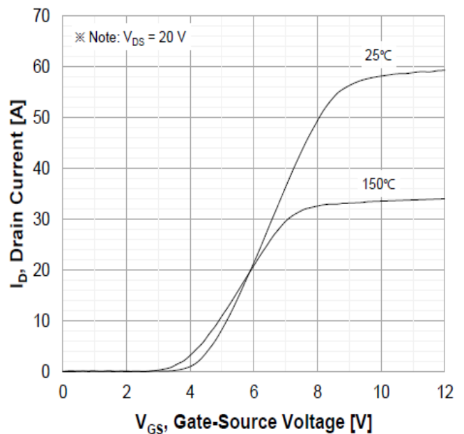
Transfer characteristics
