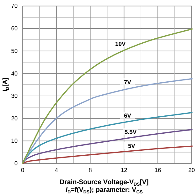
Typ. output characteristics T_j=25 °C
