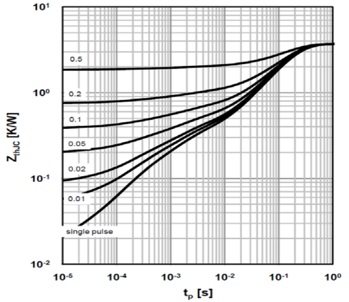
Max. transient thermal impedance TO-220FullPAK
