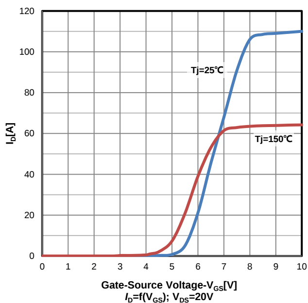
Transfer characteristics
