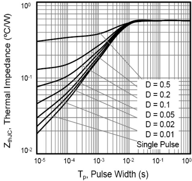
Max. transient thermal impedance TO-220, TO-247
