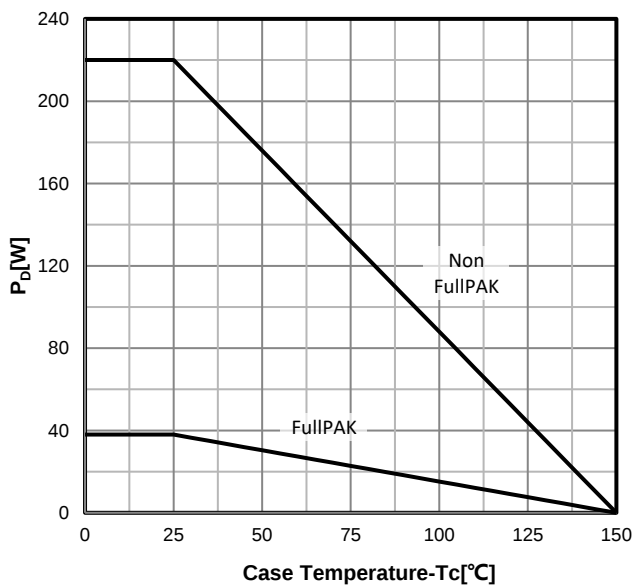
Power dissipation
