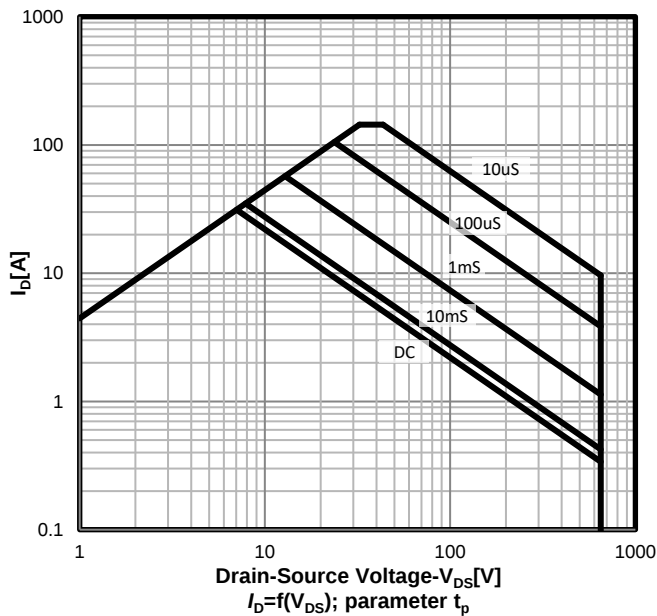
Safe operating area TC=25 °C TO-220, TO-247
