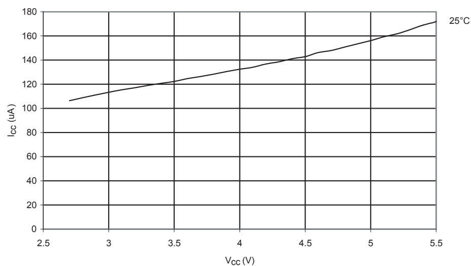
Figure 153. Active Supply Current vs. V_{CC} (External Oscillator, 32kHz)
