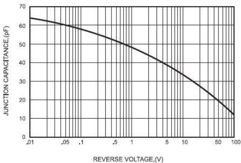
FIG.5-TYPICAL JUNCTION CAPACITANCE
