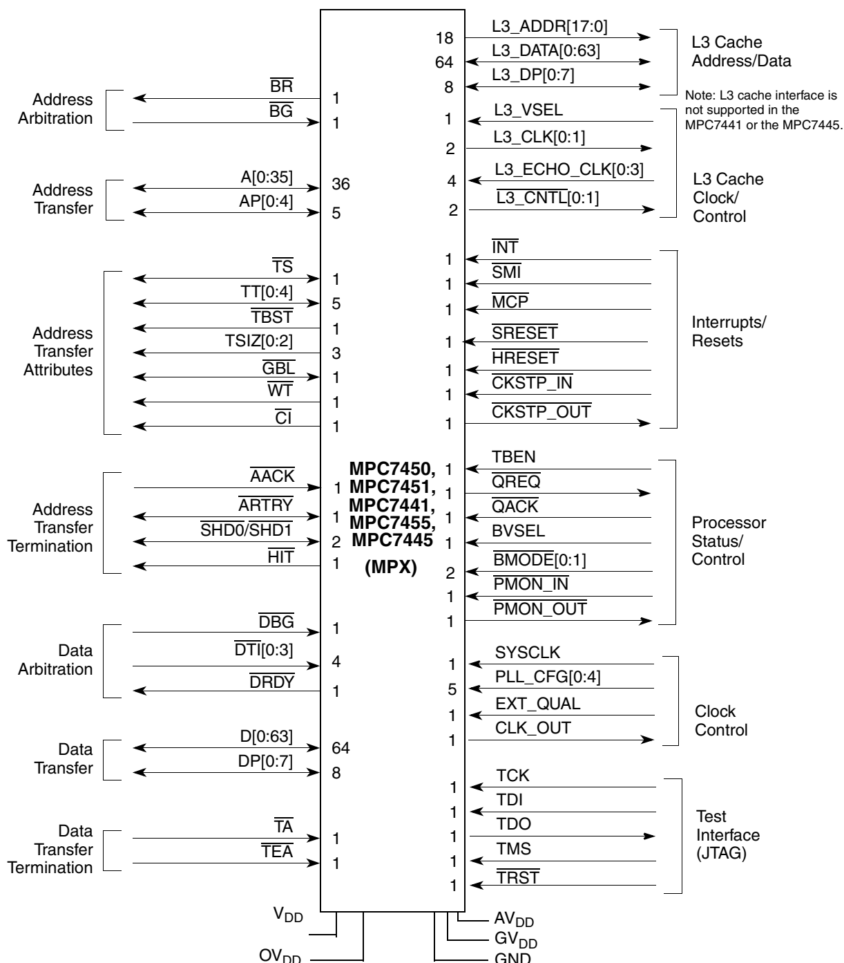
Figure 8-1. MPX Bus Signal Groups in the MPC7450, MPC7451, MPC7441, MPC7455, and MPC7445
