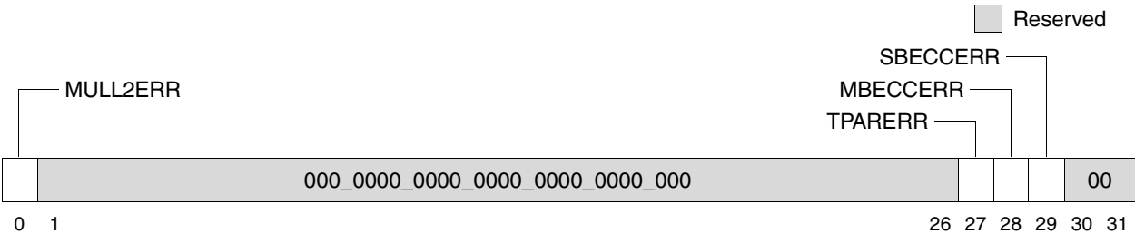
Figure 2-24. L2 Error Detect Register (L2ERRDET) for the MPC7448
