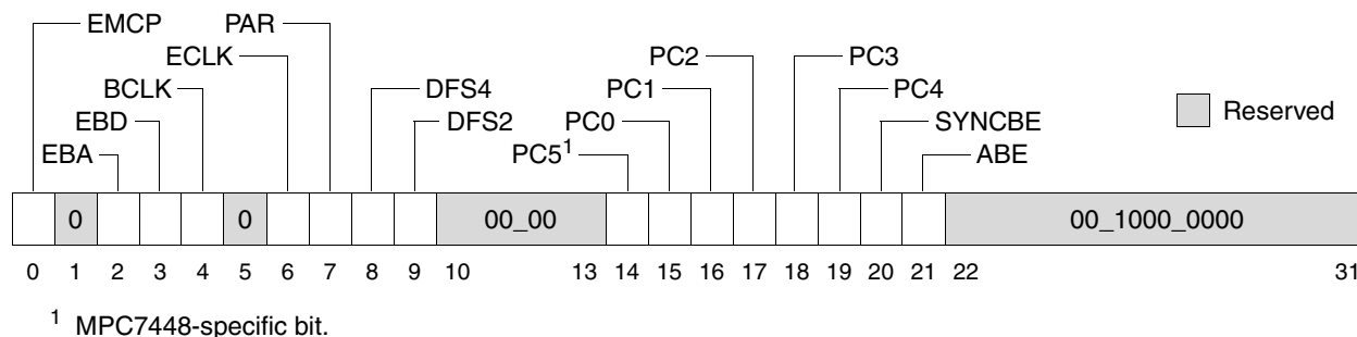
Figure 2-12. MPC7448 Hardware Implementation-Dependent Register 1 (HID1) for the MPC7448
