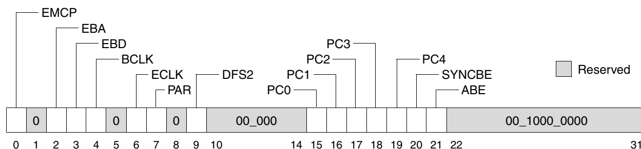
Figure 2-11. Hardware Implementation-Dependent Register 1 (HID1) for the MPC7447A
