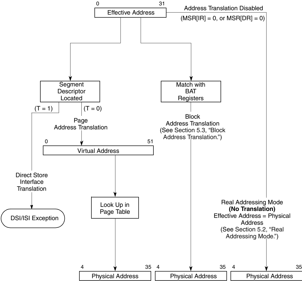
Figure 5-5. Address Translation Types for 32-Bit Physical Addressing
