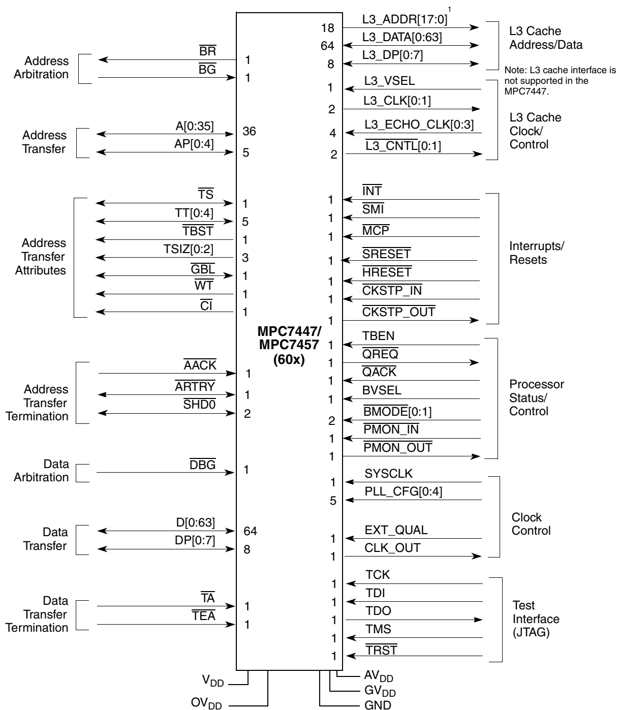
Figure 8-6. 60x Bus Signal Groups in the MPC7447 and the MPC7457
