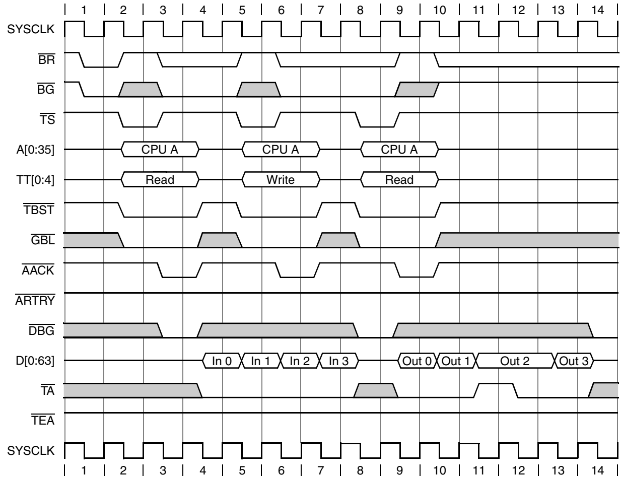
Figure 9-26. Burst Transfers with Data Delay Controls
