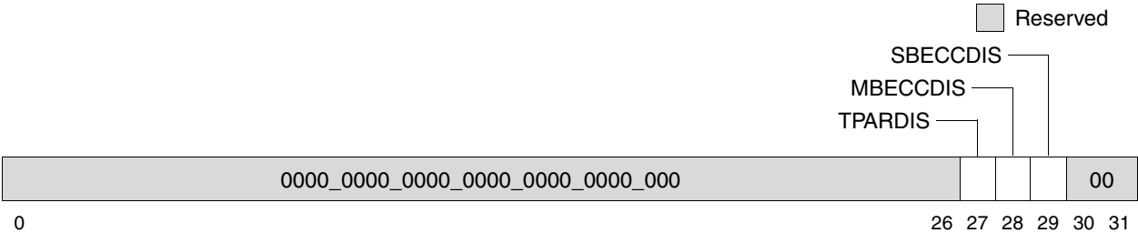
Figure 2-25. L2 Error Disable Register (L2ERRDIS) for the MPC7448
