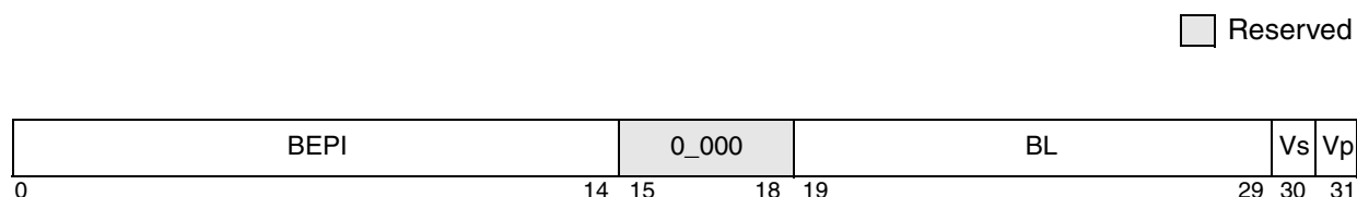
Figure 5-9. Format of Upper BAT Register (BATU)—Extended Addressing for the MPC7441, MPC7450, and MPC7451
