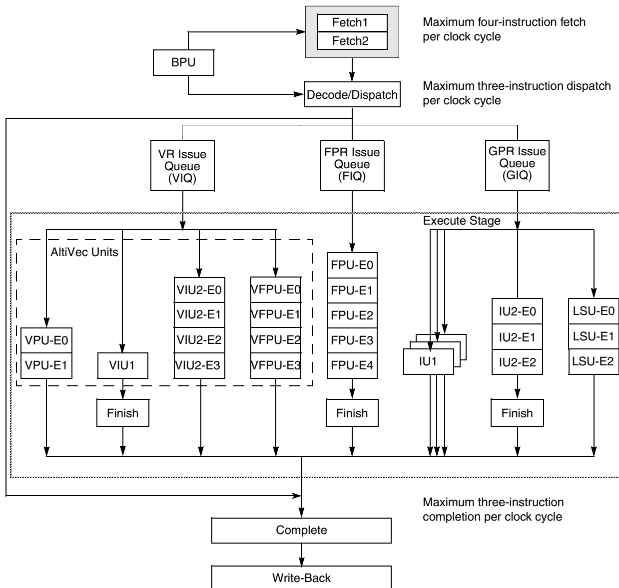
Figure 6-2. Superscalar/Pipeline Diagram
