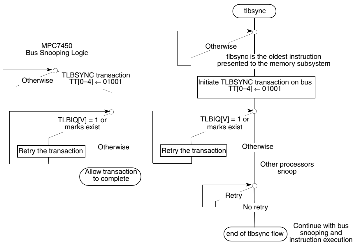
Figure 5-20. tlbsync Instruction Execution and Bus Snooping Flow
