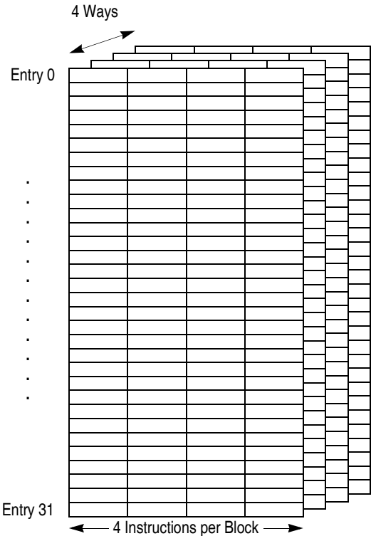
Figure 6-5. BTIC Organization
