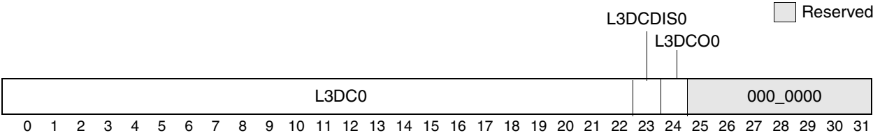
Figure 2-33. L3 Cache Control Register (L3ITCR0) for the MPC7451 and MPC7455
