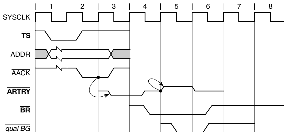
Figure 9-10. Snooped Address Cycle with \overline{ARTRY}
