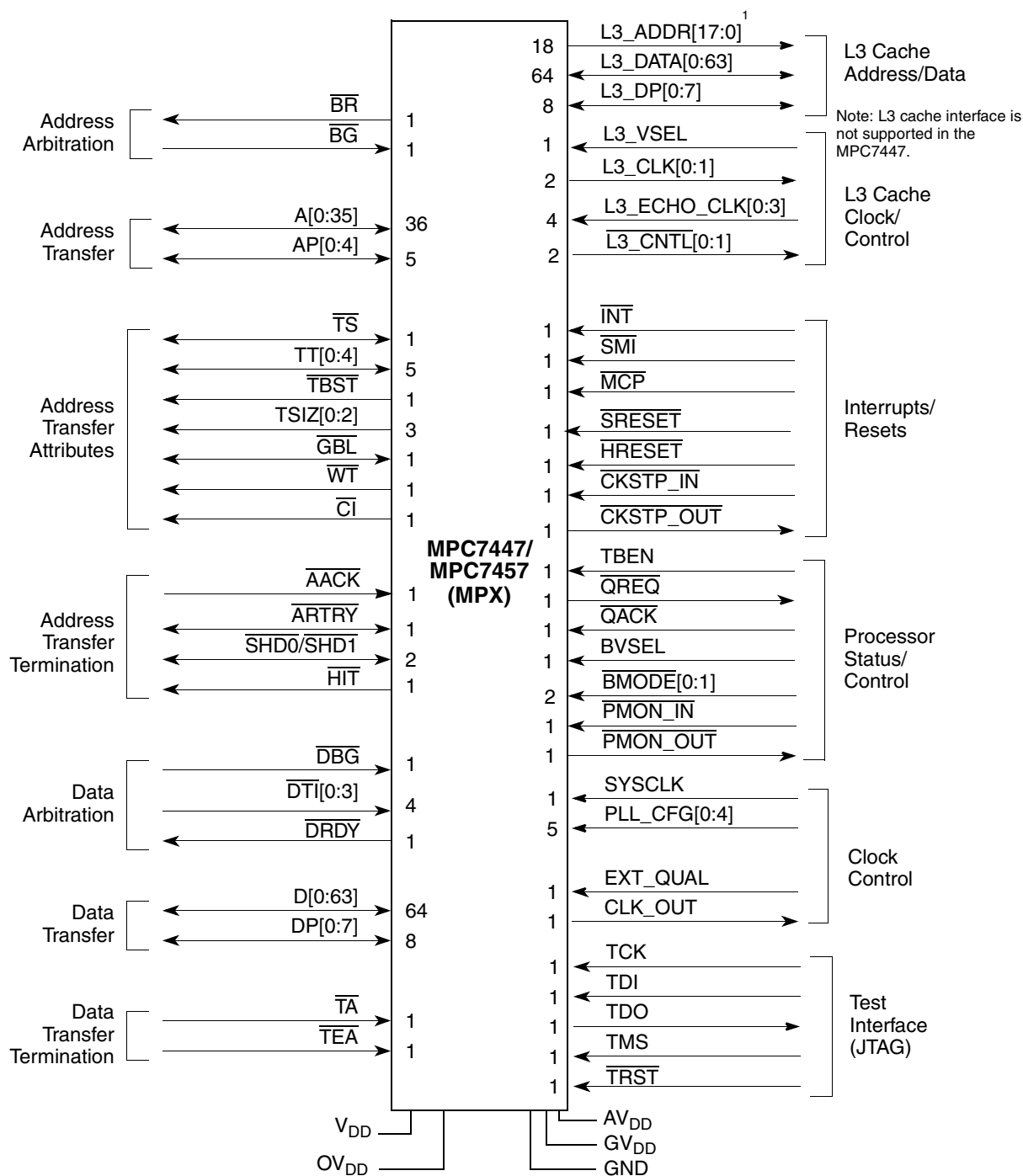
Figure 1-9. MPX Bus Signal Groups in the MPC7447 and MPC7457
