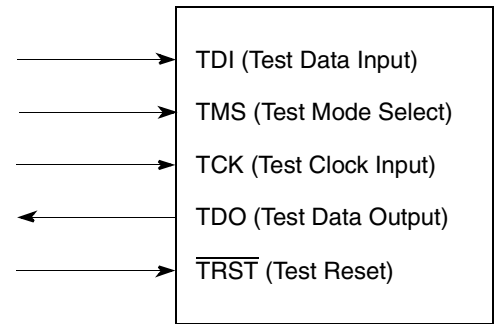
Figure 9-28. IEEE 1149.1a-1993 Compliant Boundary-Scan Interface
