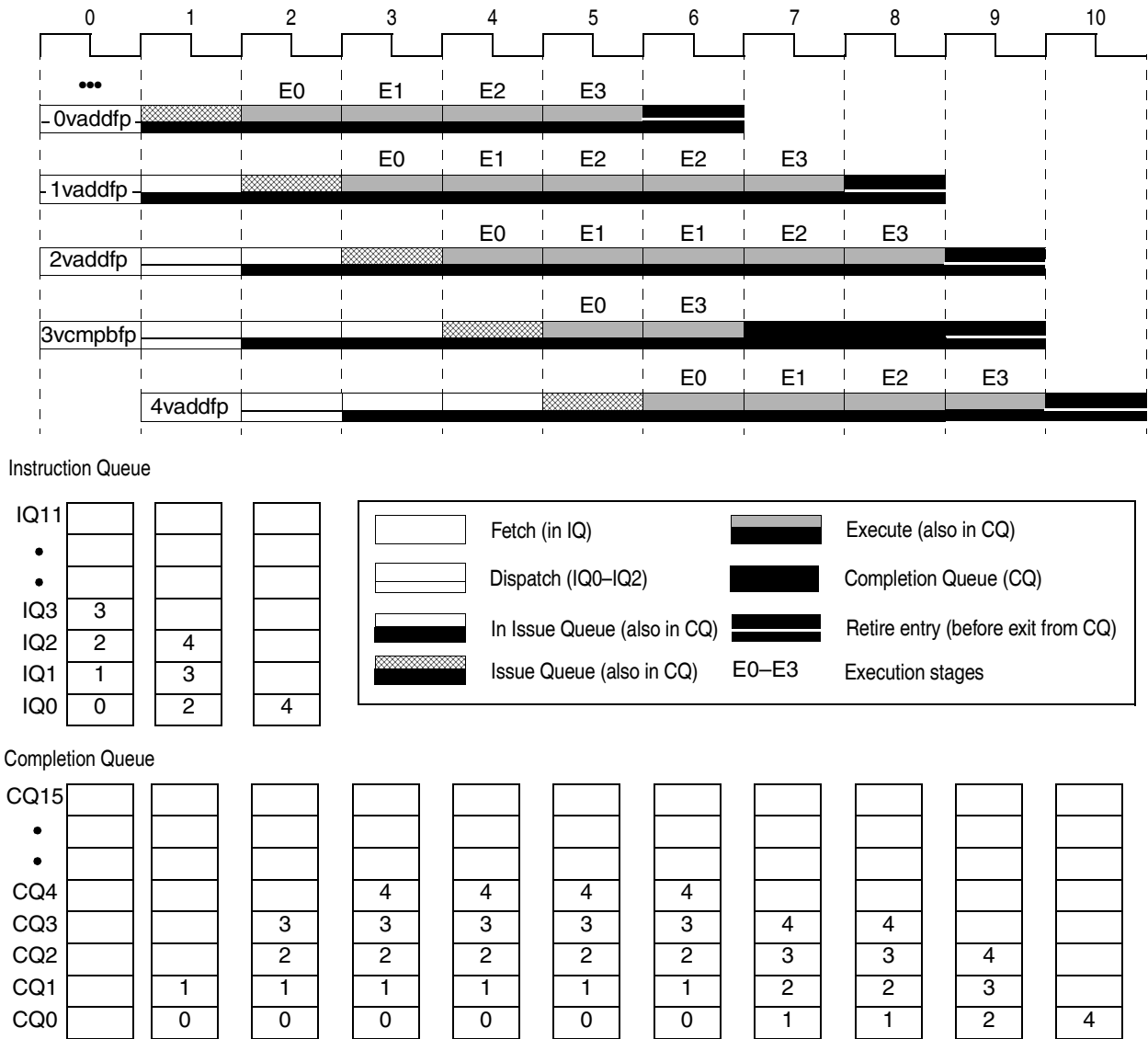
Figure 6-17. Vector Float Compare Bypass Blocking
