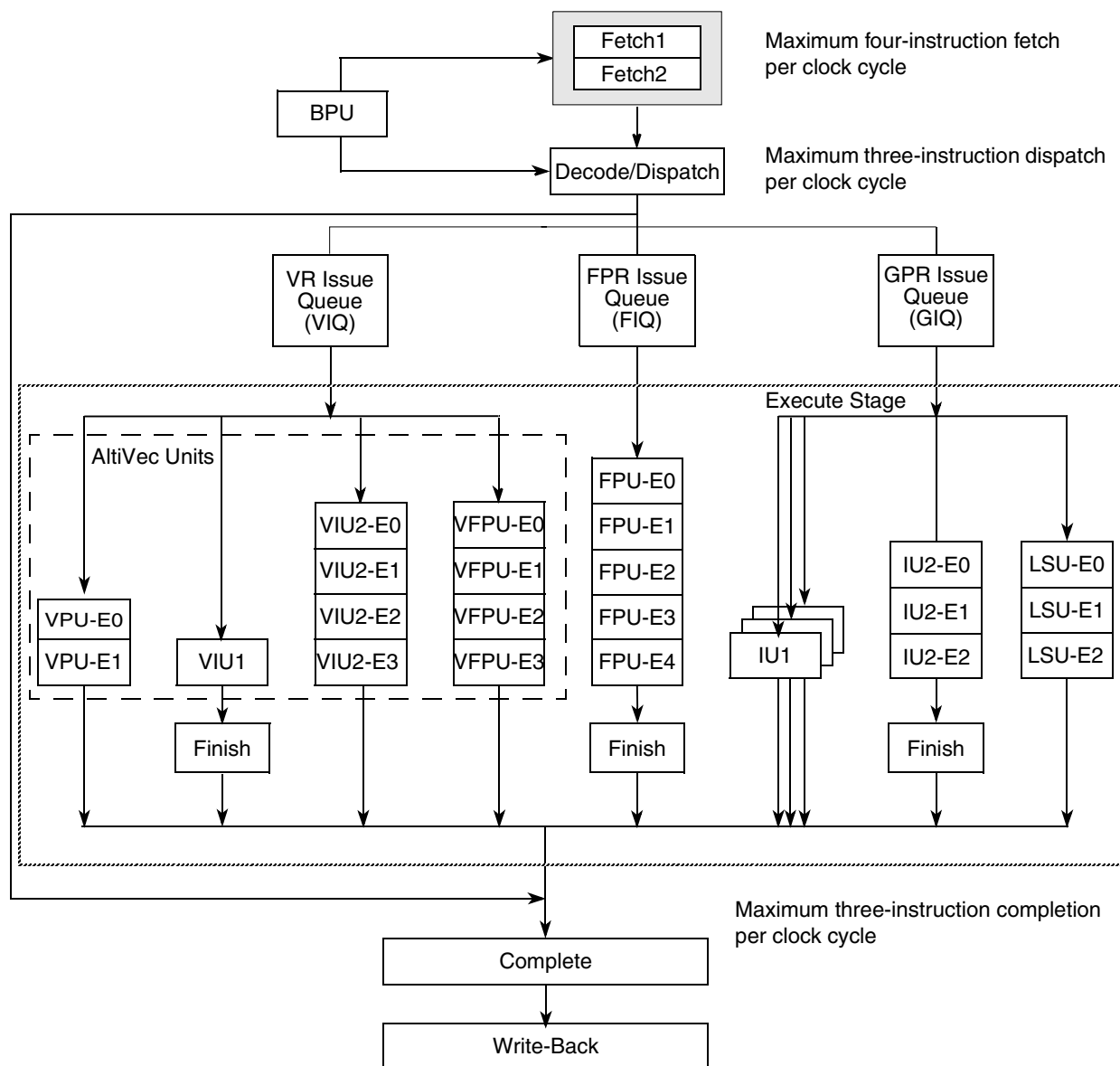
Figure 1-16. Superscalar/Pipeline Diagram
