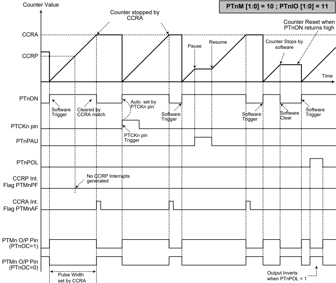
Single Pulse Output Mode (n=0)
