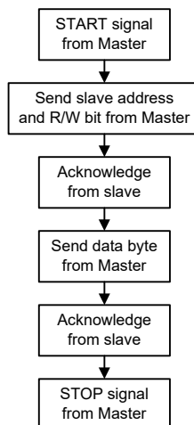
I²C Interface Operation
