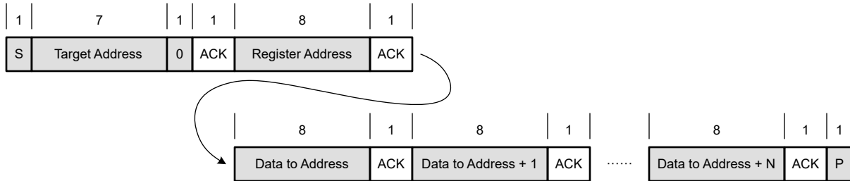
Figure 6-11. Multi-byte Write
