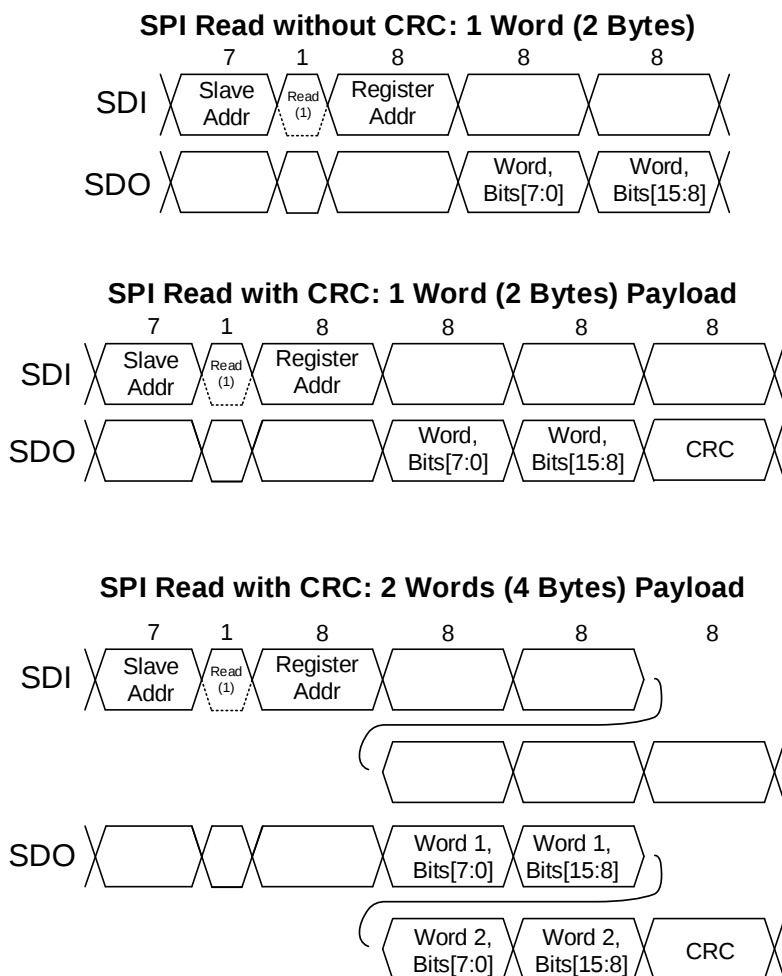
Figure 21: SPI Read Transaction
