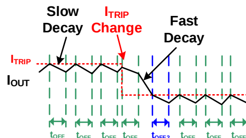
Figure 4: Slow Decay during t_{OFF} Unless I_{OUT} > I_{TRIP} at the End of t_{OFF}
