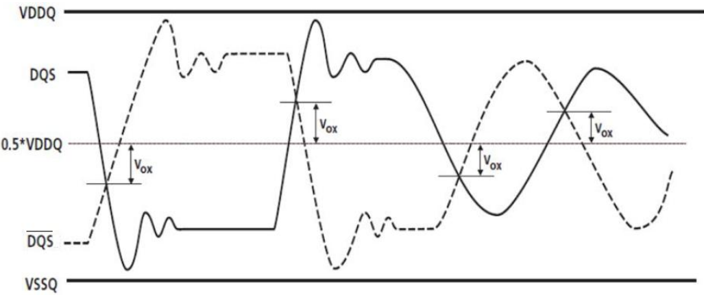
Definition of Output cross point voltage for DQS and \overline{\text{DQS}}
