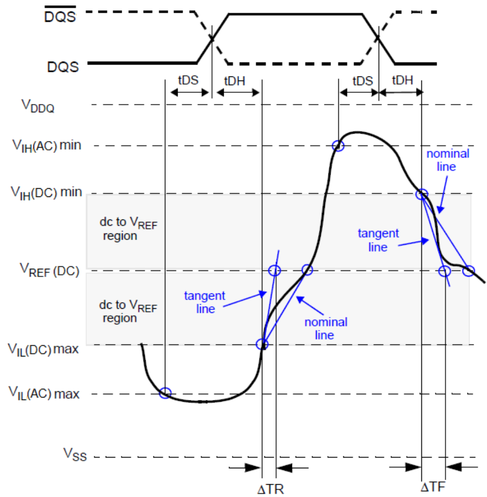
Illustration of tangent line for hold time tDH (for DQ with respect to strobe)
