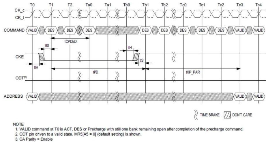
Power Down Entry and Exit Timing with C/A Parity
