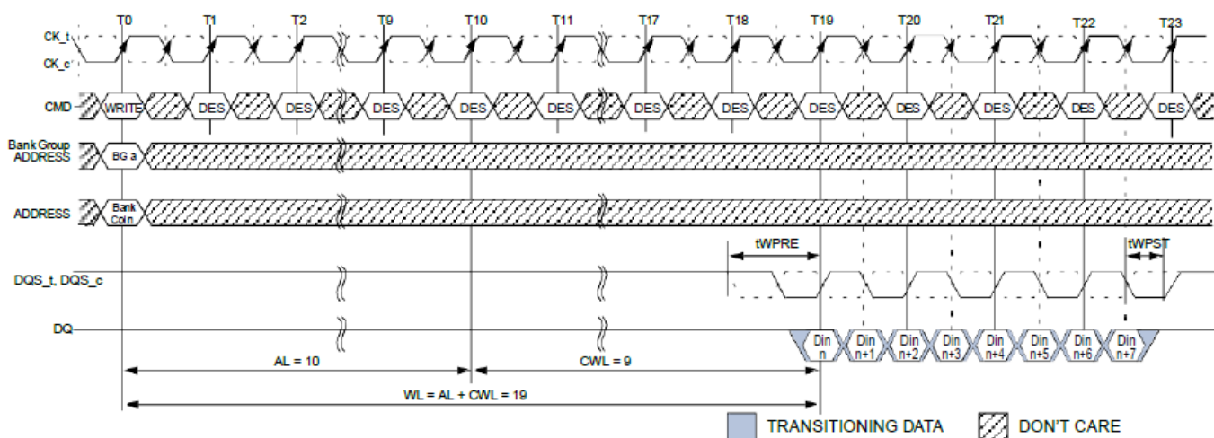
WRITE Burst Operation WL = 19 (AL = 10, CWL = 9, BL8)
