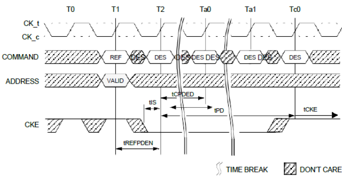
Refresh Command to Power-Down Entry
