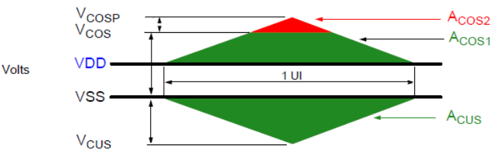
Clock Overshoot and Undershoot Definition
