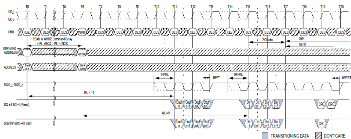
READ (BC4:Fixed) to WRITE (BC4:Fixed) with 1tCK Preamble and Write CRC in Same or Different Bank Group
