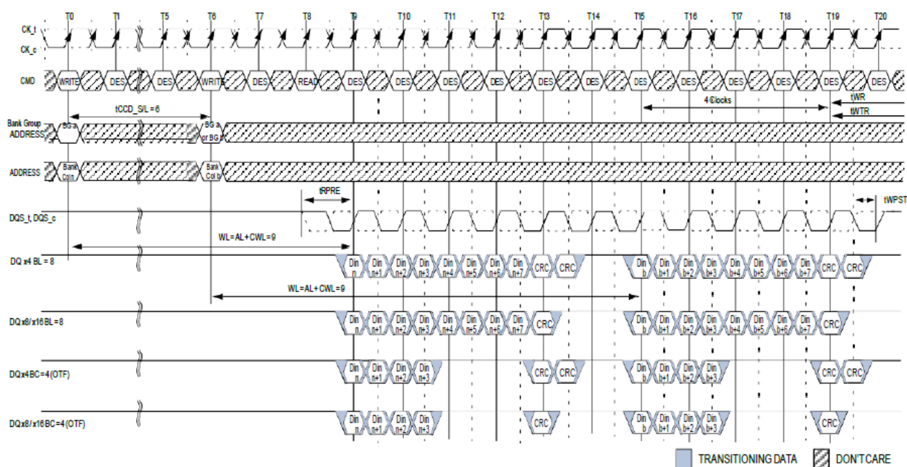
Nonconsecutive WRITE (BL8/BC4) OTF with 1tCK Preamble and Write CRC in Same or Different Bank Group
