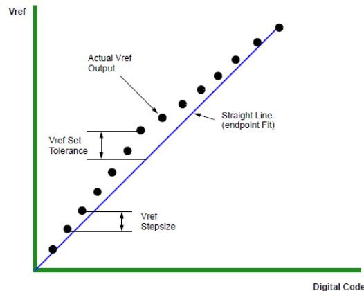
Example of Vref set tolerance(max case only shown) and stepsize
