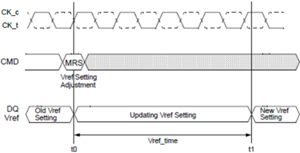
Vref_time timing diagram
