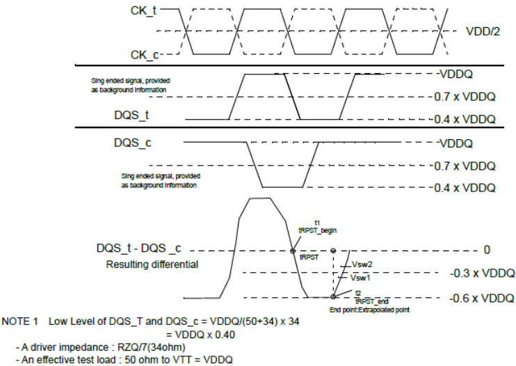
Method for calculating tRPST transitions and endpoints
