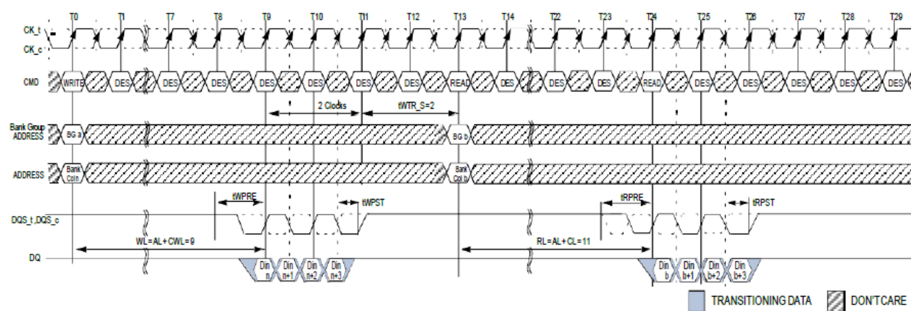
WRITE (BC4) Fixed to READ (BC4) Fixed with 1tCK Preamble in Different Bank Group
