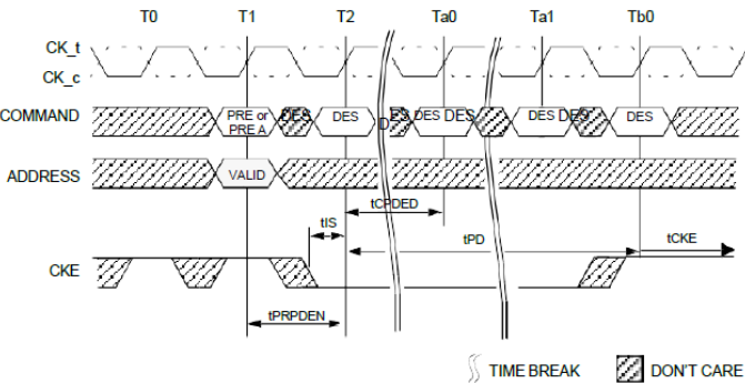
Precharge/Precharge all Command to Power-Down Entry
