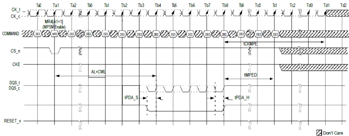
Maximum Power Saving mode Entry with PDA
