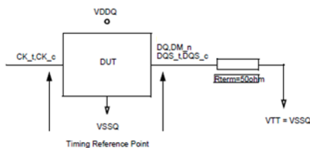
ODT Timing Reference Load
