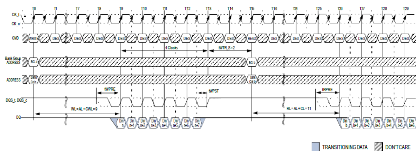
WRITE (BL8) to READ (BL8) with 1tCK Preamble in Different Bank Group
