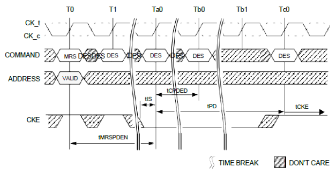
MRS Command to Power-Down Entry
