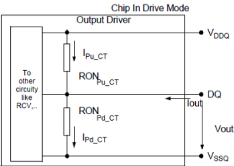
Output Driver
