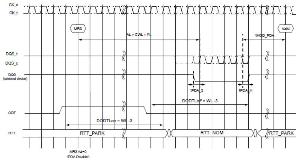
MRS w/ per DRAM addressability (PDA) Exit
