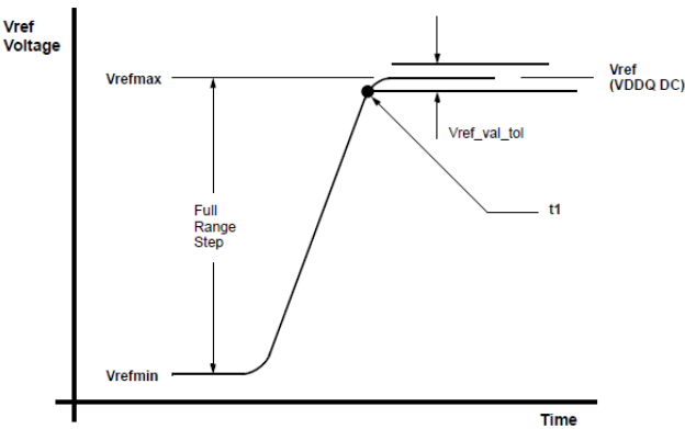
Vref full step from Vrefmin to Vrefmax case
