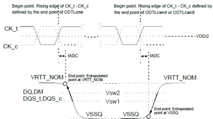
Definition of tADC at Dynamic ODT Control
