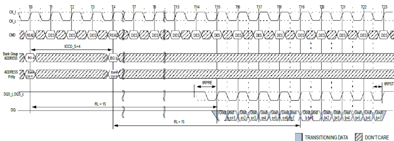
Consecutive READ (BL8) with 1tCK Preamble and CA Parity in Different Bank Group
