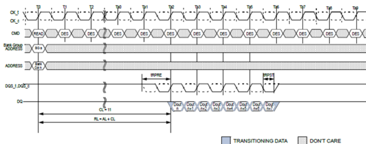
READ Burst Operation RL = 11 (AL = 0, CL = 11, BL8)
