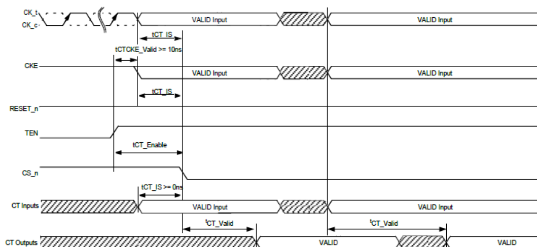
Timing Diagram for Connectivity Test(CT) Mode
