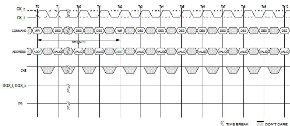
MPR Back to Back Write Timing
