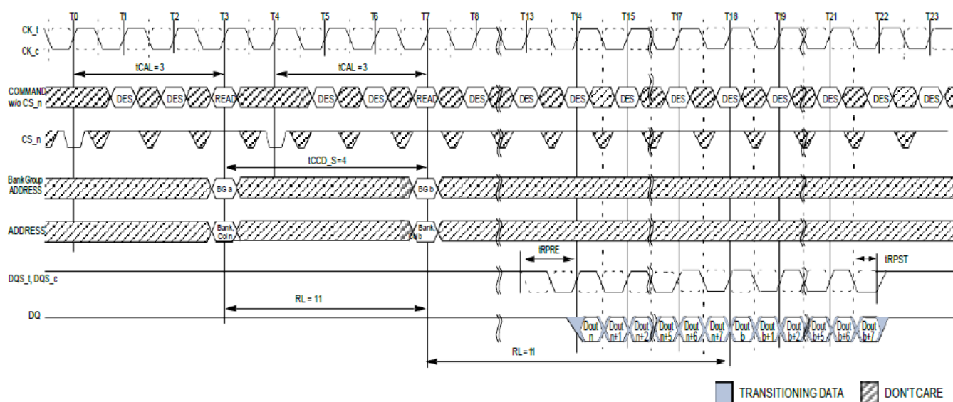
Consecutive READ (BL8) with CAL(3) and 1tCK Preamble in Different Bank Group
