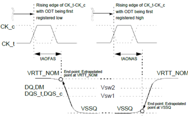
Definition of t_{AOFAS} and t_{AONAS}
