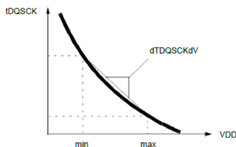
TDQSCKTdV Definition
