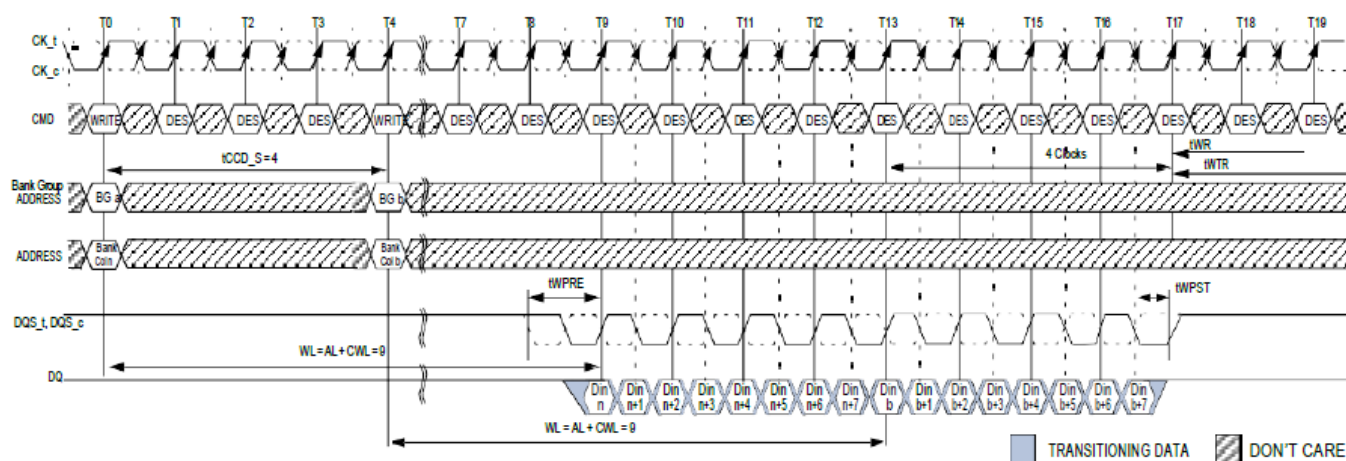
Consecutive WRITE (BL8) with 1tCK Preamble in Different Bank Group
