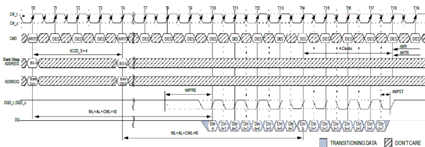
Consecutive WRITE (BL8) with 2tCK Preamble in Different Bank Group
