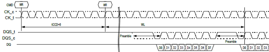
2tCK mode
