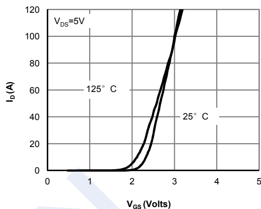
Figure 2: Transfer Characteristics (Note 6)
