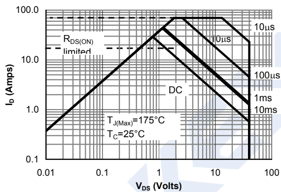
Figure 9: Maximum Forward Biased Safe Operating Area
