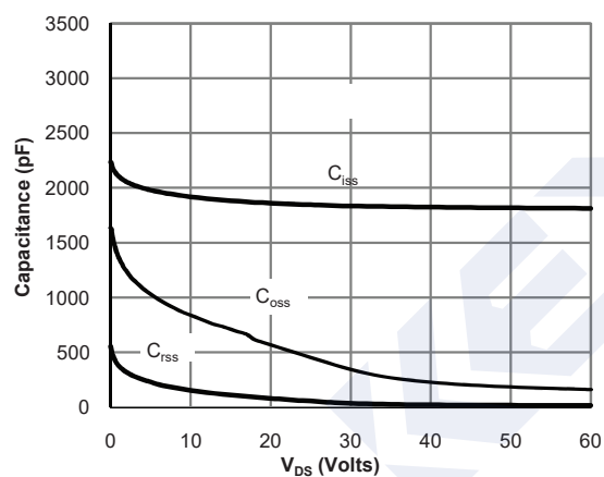
Figure3. Capacitance Characteristics
