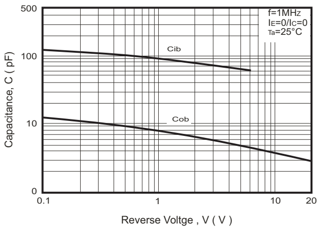
Fig. 5 - Cob/Cib - VCB/VEB
