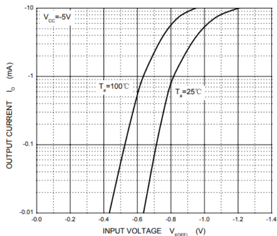
Fig 2: OFF Characteristics
