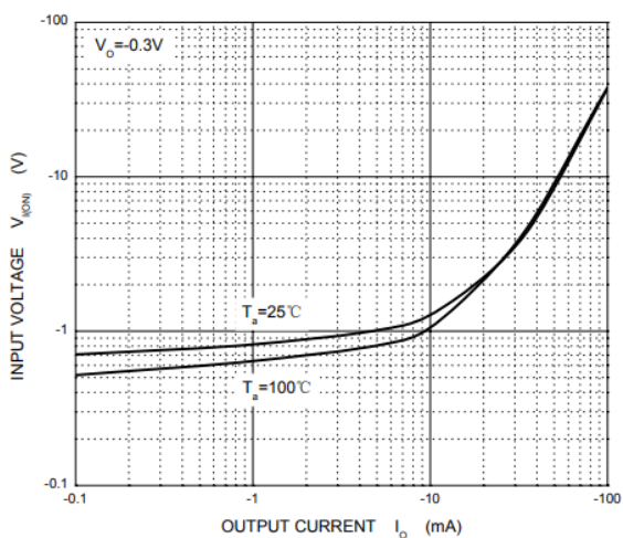
Fig 1: ON Characteristics
