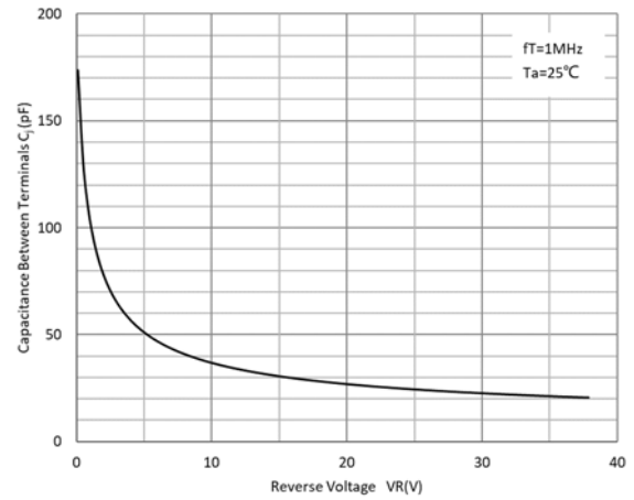
Fig 2: Capacitance Capability
