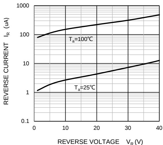
Reverse Characteristics
