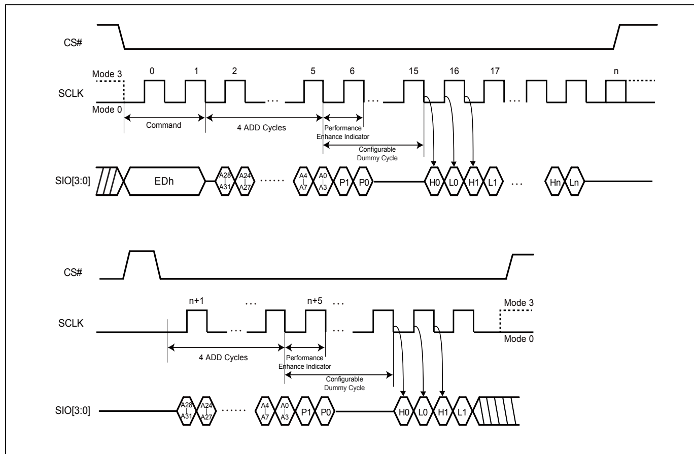
Figure 46. 4 x I/O DT Read Performance Enhance Mode Sequence (QPI Mode)
