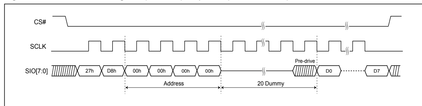
Figure 99. Read Password Register (RDPASS) Sequence (STR-OPI Mode)
