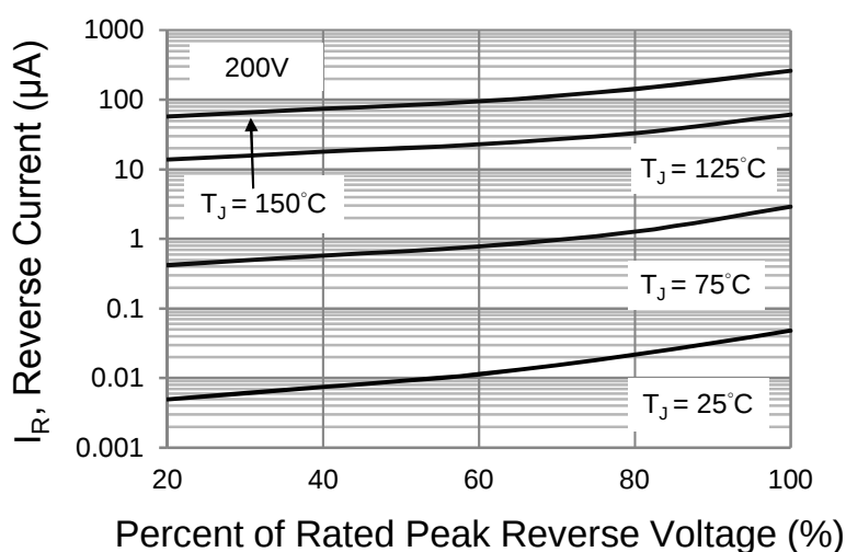
Fig.5 Typical Reverse Characteristics
