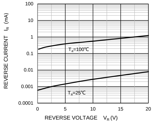
Reverse Characteristics
