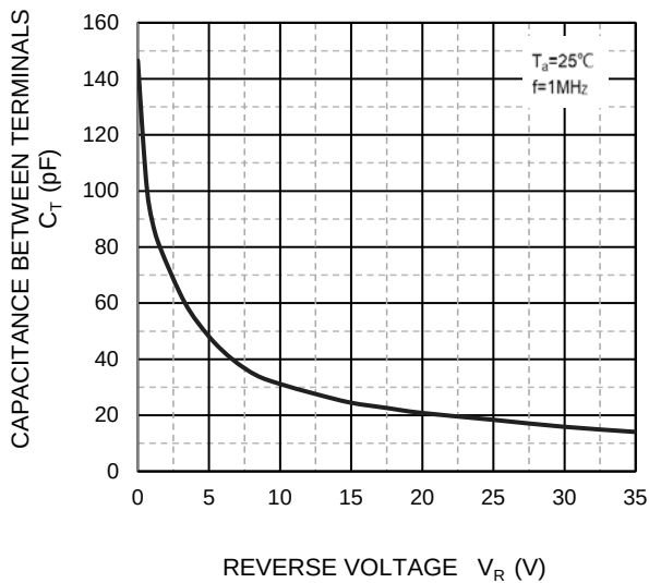
Capacitance Characteristics
