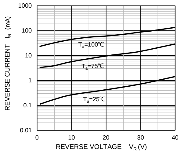
Reverse Characteristics
