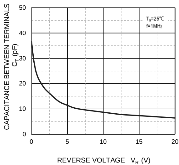
Capacitance Characteristics Per Diode
