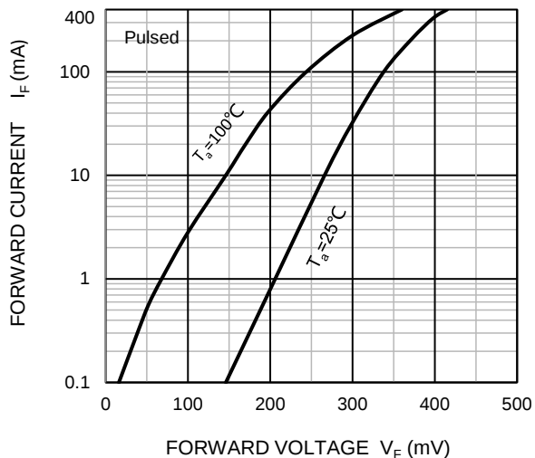
Forward Characteristics
