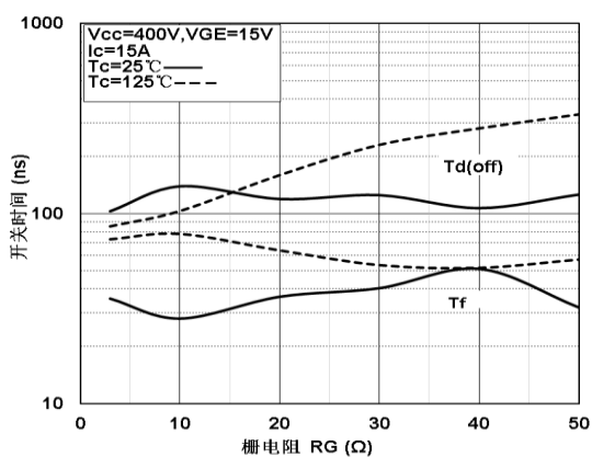
Figure 9. Switching Time - R_g Characteristics
