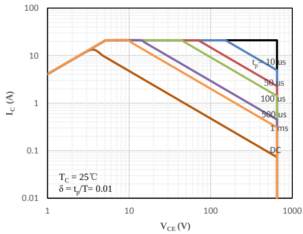
Fig 13 SOA characteristics
