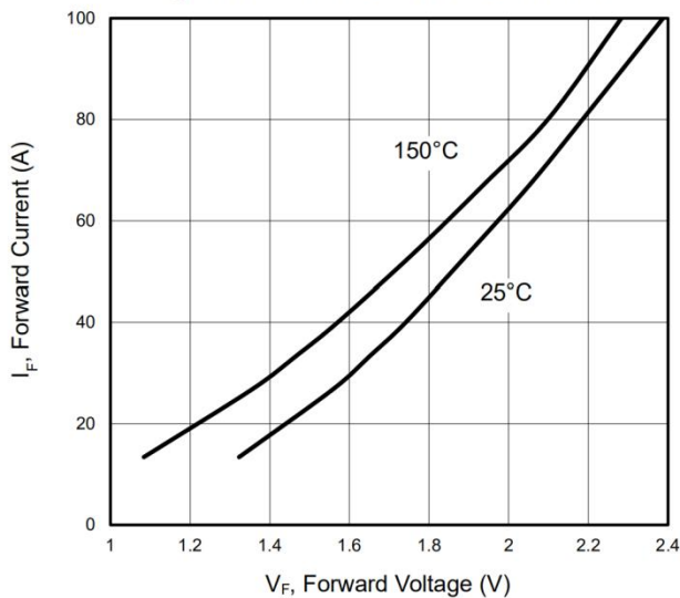
Figure 7 Forward Characteristics
