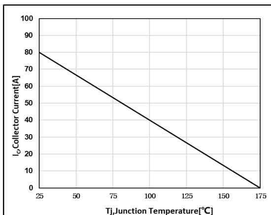
Figure 16.Collector Current-Tj Characteristics
