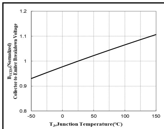
Figure 19. Breakdown Voltage vs Junction Temperature
