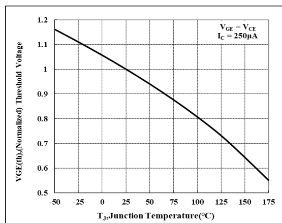
Figure 20. Threshold Voltage vs Junction Temperature
