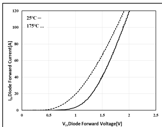
Figure 15.Diode Forward Characteristics
