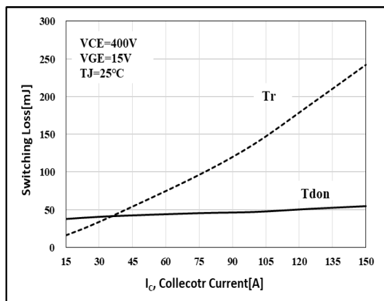
Figure 13.Switching Time-Ic Characteristics
