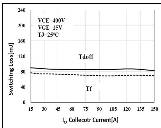
Figure 14.Switching Time-Ic Characteristics
