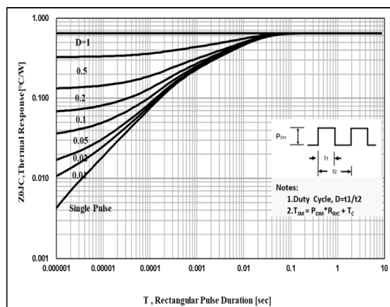
Figure 22. IGBT Transient Thermal Impedance
