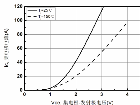
Figure 3. Saturation Voltage Characteristics
