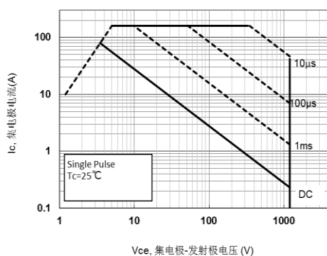
Figure 17. Forward Bias Safe Operating Area
