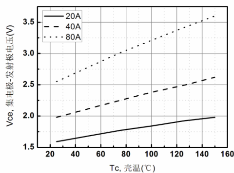
Figure 4. Saturation Voltage - T_c Characteristics
