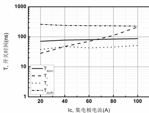
Figure 13. Switching Time-Ic Characteristics
