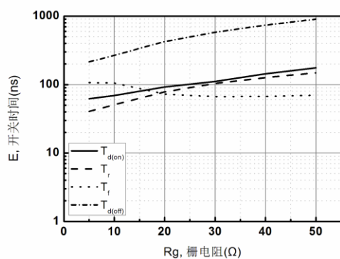
Figure 9. Switching Time- R_g Characteristics
