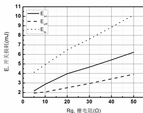
Figure 8. Switching Loss- R_g Characteristics
