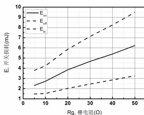
Figure 6. Switching Loss- R_g Characteristics
