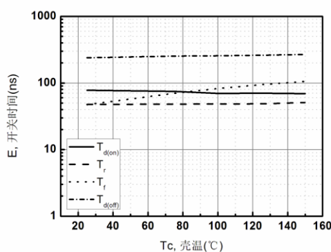
Figure 11. Switching Time- T_c Characteristics
