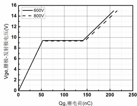
Figure 14. Gage Charge Characteristics
