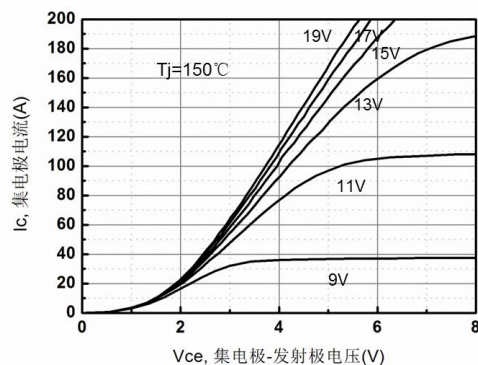
Figure 2. Output Characteristics
