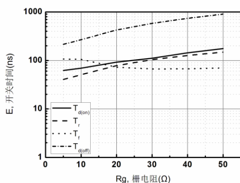
Figure 7. Switching Time- R_g Characteristics
