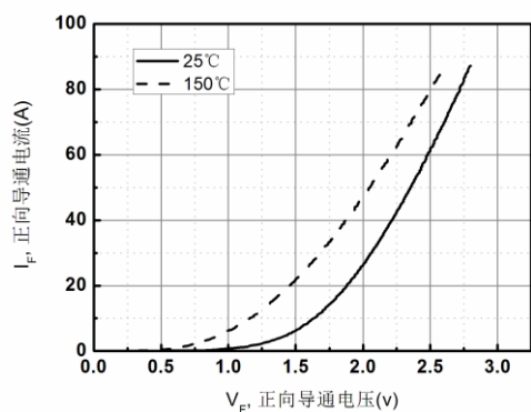
Figure 15. Diode Forward Characteristics
