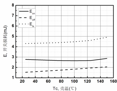
Figure 10. Switching Loss- T_c Characteristics
