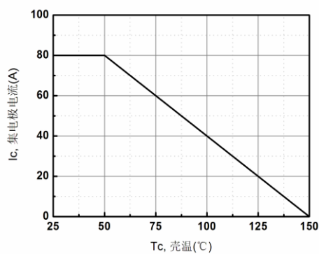
Figure 16. Collector Current-Tc Characteristics
